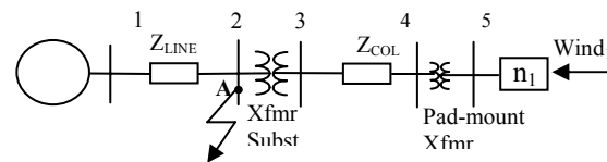
Figure 5. A typical single line diagram of a wind farm power system with a single turbine
