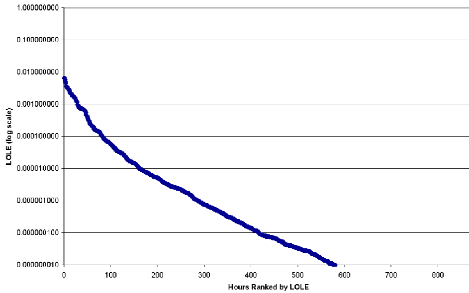
FIGURE 3. LOLP DURATION CURVE.
