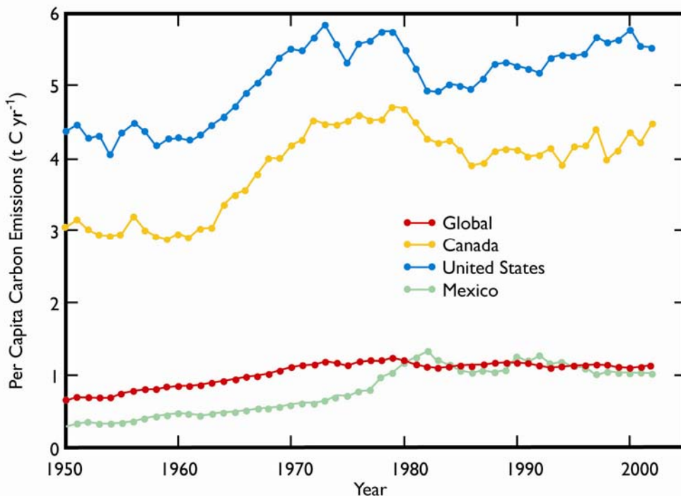
Fig. 8. Per capita emissions of CO 2 from fossil-fuel consumption (and cement manufacture) in the United States, Canada, and Mexico and for the global total of emissions. Source: Marland et al., 2005.
