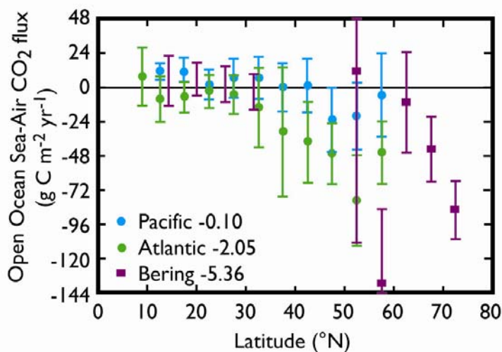
Figure 15-4. Estimated air-sea CO 2 fluxes (grams of carbon per square meter per year) from 550,000 seawater CO 2 partial pressure (pCO 2 ) observations made from 1979 to 2004 in ocean waters surrounding the North American continent. (A) Waters within one degree (about 80 km) of the coast and (B) open ocean waters between 300 and 900 km from the shore (see Figure 15-3B). The annual mean air-sea pCO 2 difference (delta pCO 2 ) values were calculated from the weekly mean atmospheric CO 2 concentrations in the GLOBALVIEW-CO 2 database (2004) over the same pixel area in the same week and year as the seawater pCO 2 was measured. The monthly net air-sea CO 2 flux was computed from the mean monthly wind speeds in the National Centers for Environmental Prediction/National Center for Atmospheric Research (NCEP/NCAR) database in the (wind speed) 2 formulation for the air-sea gas transfer rate by Wanninkhof (1992). The ± uncertainties represent one standard deviation.
