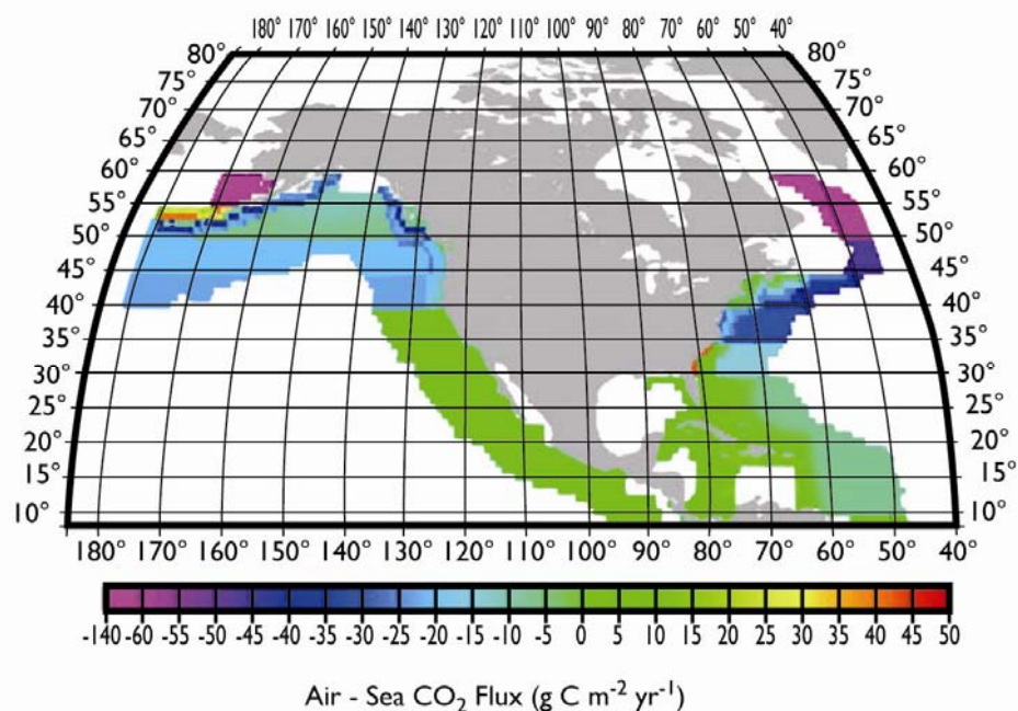
Figure 15-3. (A). Distribution of coastal surface water CO 2 partial pressure measurements made between 1979 and 2004. (B). The distribution of the annual mean air-sea net CO 2 flux over 1° × 1° pixel areas (N-S 100 km, E-W 80 km) around North America. The flux (grams of carbon per square meter per year) represents the climatological mean over the 25-year period. The magenta-blue colors indicate that the ocean water is a sink for atmospheric CO 2 , and the green-yellow-orange colors indicate that the sea is a CO 2 source. The data were obtained by the authors and collaborators of this chapter and are archived at the Lamont-Doherty Earth Observatory ( www.ldeo.columbia.edu/res/pi/CO2 ).
