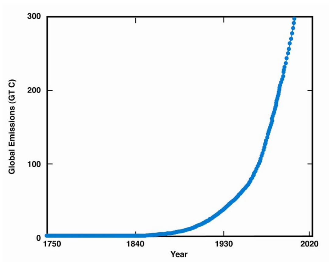
Fig. 1. Cumulative global emissions of CO 2 from fossil-fuel combustion and cement manufacture from 1751 to 2002. Source data: Marland et al., 2005.
