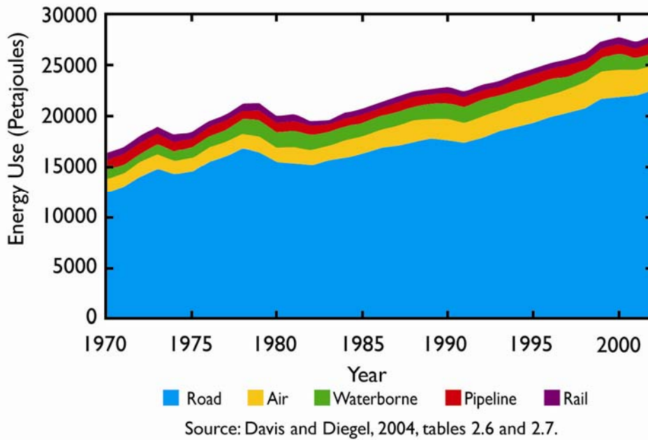
Fig. 7-5B. Evolution of transport energy use in the United States.
