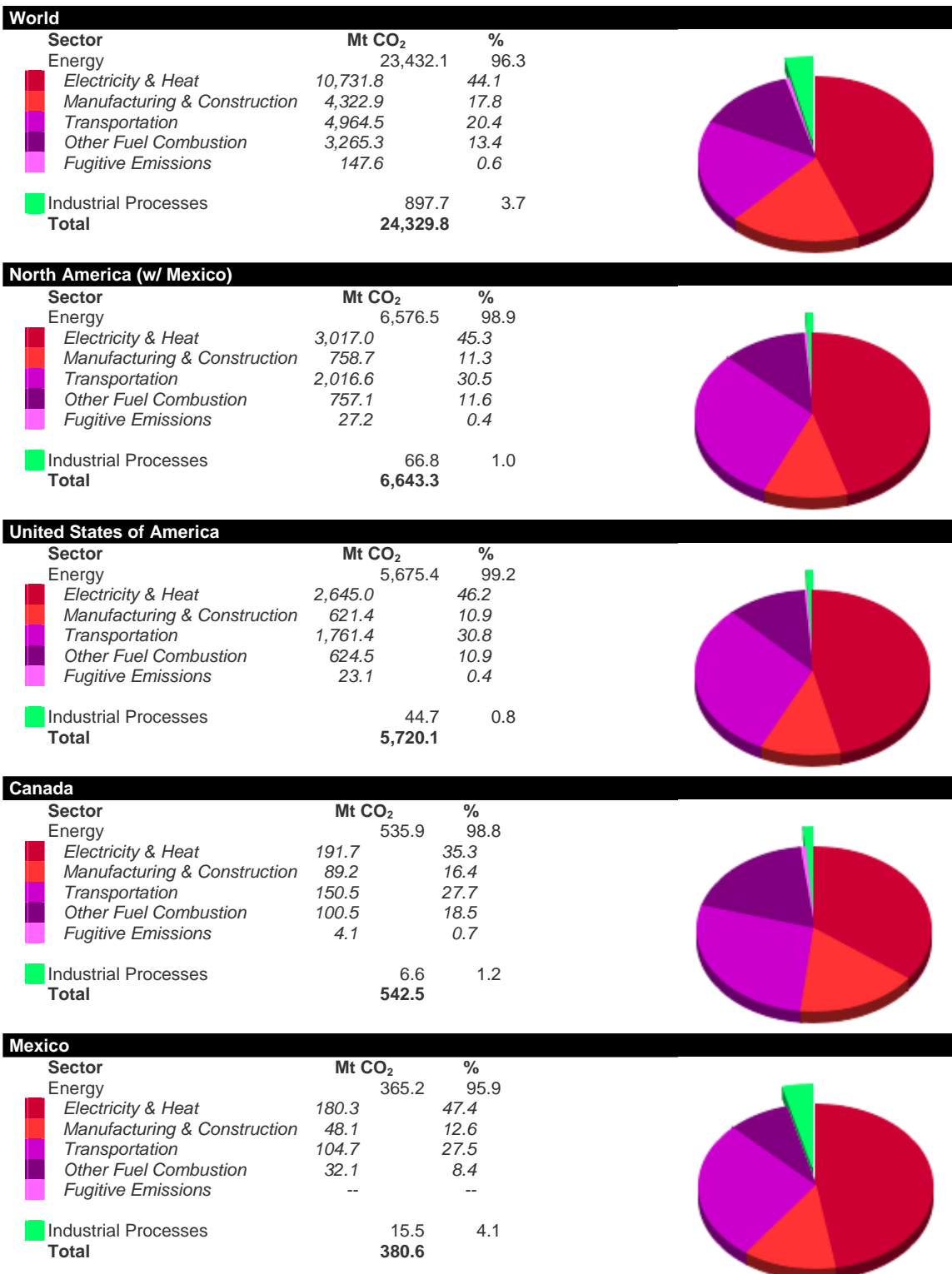
Fig. 8-1A. CO 2 emissions by sector in 2002. Source: WRI (World Resources Institute), 2005. The magnitude and/or range of uncertainty for the given numerical values is not provided in the reference. To convert from Mt CO 2 to Mt C, multiply the Mt CO 2 value by 12/44.
