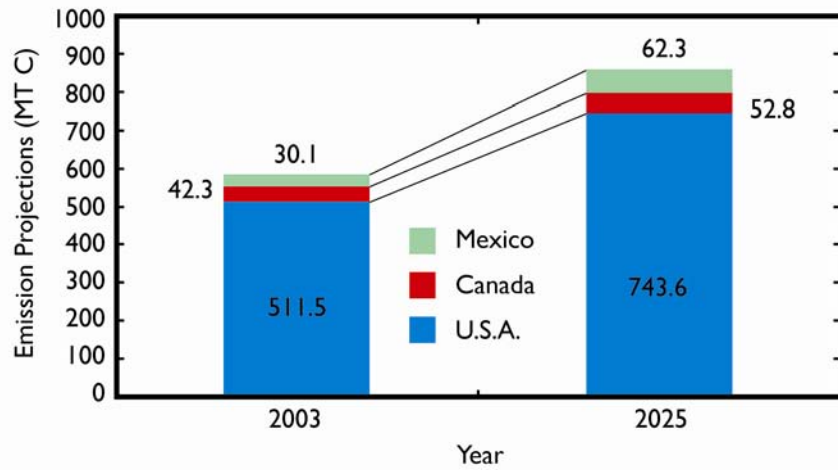
Fig. 7-7. Projected carbon dioxide emissions from the North American transport sector in 2025, based on EIA IEO 2005 reference case. Source: U.S. DOE/EIA, 2005b.
