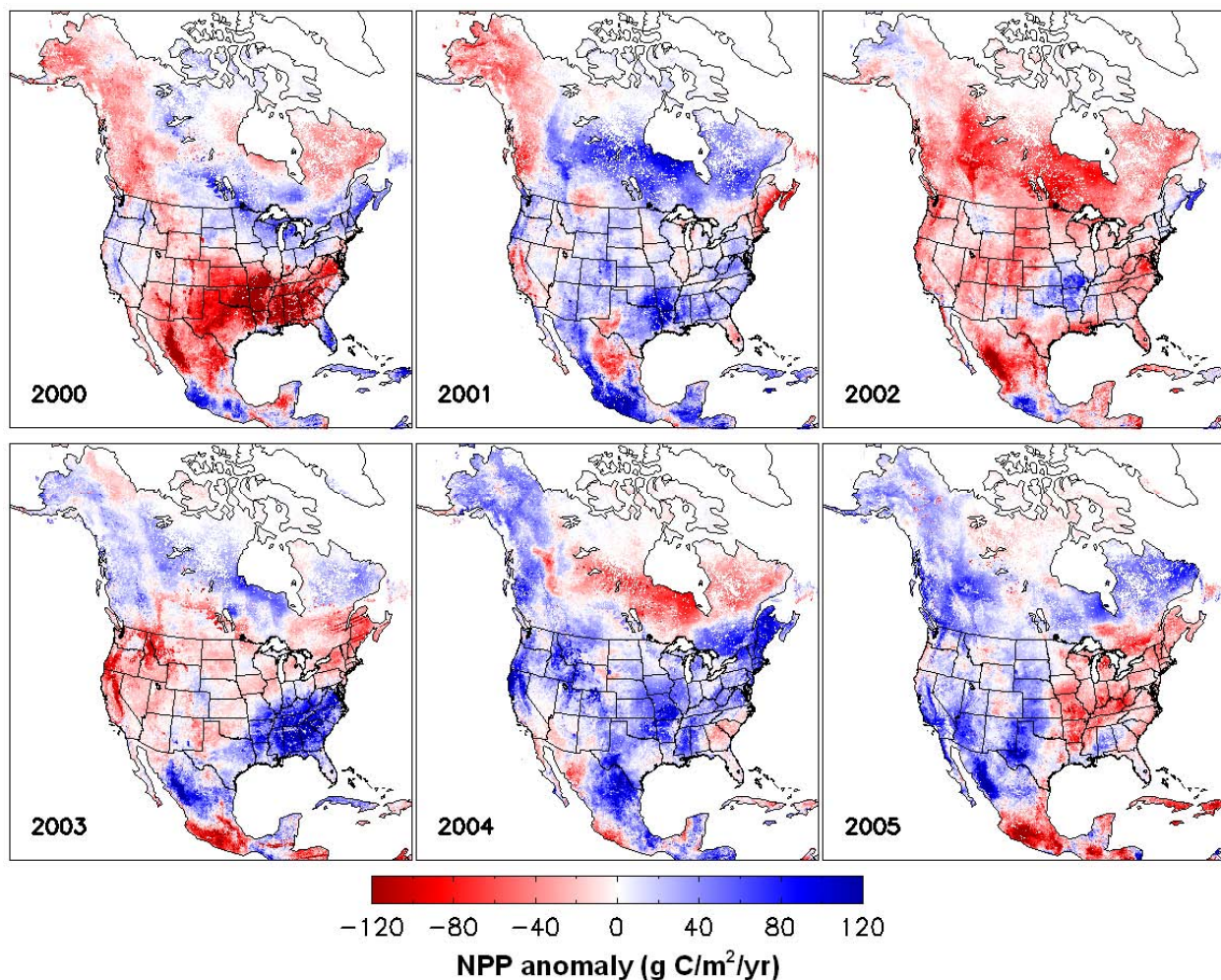
Figure 1-2. Variability in net primary production (NPP) for North America from 2000-2005. Values are the deviation from 6-year average annual net primary production (NPP) estimated by the MOD17 1-km resolution data product from the Moderate Resolution Imaging Spectroradiometer (MODIS) aboard NASA's Terra and Aqua satellites. Blue indicates regions where that year's NPP, the net carbon fixed by vegetation from the atmosphere, was greater than average; red indicates where annual NPP was less than the average. See Running et al. (2004) for further information on the MODIS NPP product. Figure courtesy of Dr. Steven W. Running, University of Montana.
