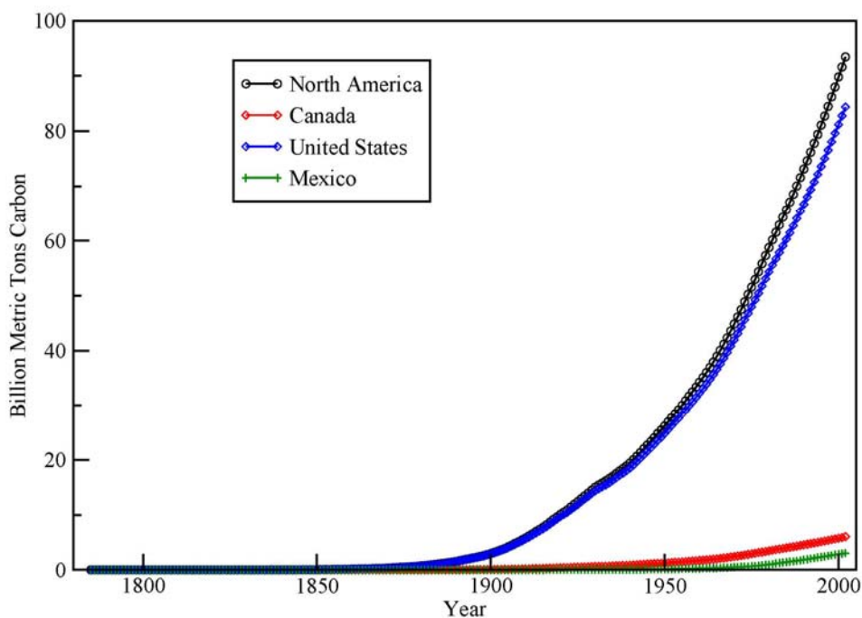
Fig. 3. The cumulative total of CO 2 emissions from fossil-fuel consumption and cement manufacture, as a function of time, for the three countries of North America and for the sum of the three. Source: Marland et al. , 2005.
