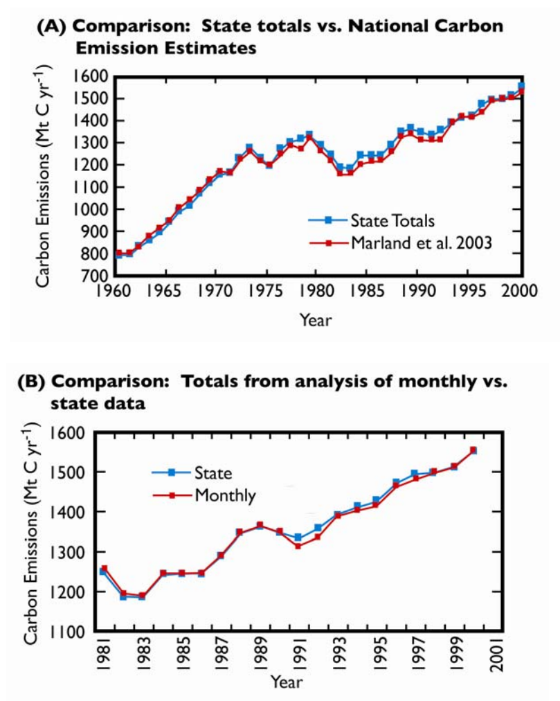
Fig. 6. A comparison of three different estimates of national annual emissions of CO 2 from fossil-fuel consumption in the United States. (6A) Estimates from U.S. Department of Energy data on fuel consumption by state (blue squares) vs. estimates based on UN Statistics Office data on apparent fuel consumption for the full United States (red squares). Source: Marland et al. , 2003. (6B) Estimates based on DOE data on fuel consumption in the 50 U.S. states (blue squares) vs. estimates based on national fuel consumption for each of the 12 months (red squares). The state and monthly data include estimates of oxidation of non-fuel hydrocarbon products; the UN-based estimates do not. Source: Blasing et al. , 2005b.
