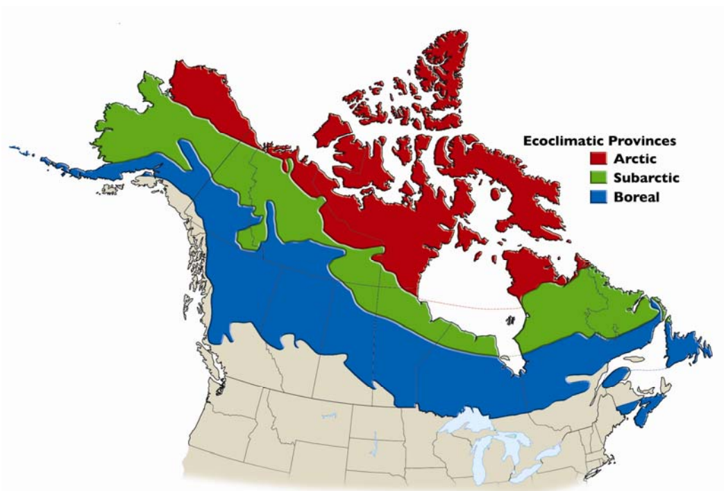
Fig. 12-2. Arctic, Subarctic, and Boreal ecoclimatic provinces (ecological regions) in North America Sources: Ecoregions Working Group, 1989; Baily and Cushwa, 1981.
