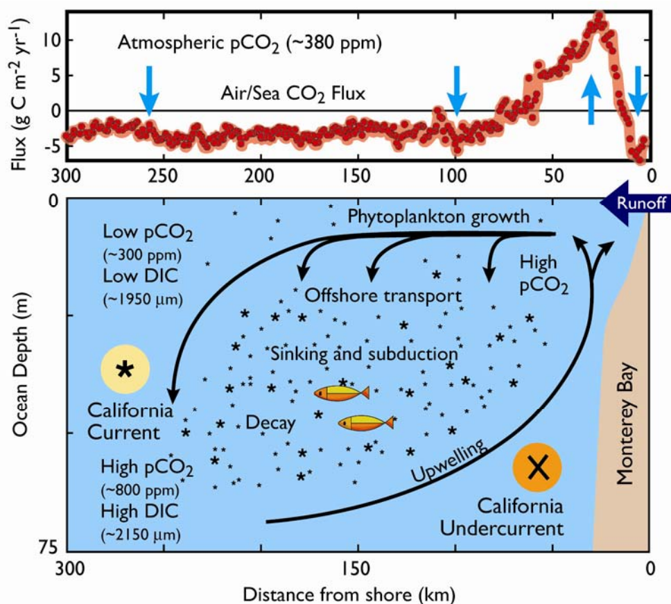
Figure 15-2. Mean air-sea CO 2 flux as calculated from shipboard measurements on a line perpendicular to the central California coast (top panel). Flux within Monterey Bay (~0-20 km offshore) is into the ocean, flux across the active upwelling region (~20-75 km offshore) is from the ocean, and flux in the California Current (75-300 km) is on average into the ocean. These fluxes result from the processes shown in the bottom panel. California Undercurrent water, which has a high CO 2 partial pressure, upwells near shore, and is advected offshore into the California Current and into Monterey Bay. Phytoplankton growing in the upwelled water use CO 2 as a carbon source, and CO 2 is drawn to low levels in those areas. Phytoplankton carbon eventually sinks or is subducted below the euphotic zone, where it decays, elevating the CO 2 levels of subsurface waters. Where the level of surface CO 2 is higher than the level of atmospheric CO 2 , diffusion drives CO 2 into the atmosphere. Conversely, where the level of surface CO 2 is lower than that of atmospheric CO 2 , diffusion drives CO 2 into the ocean. The net air-sea flux on this spatial scale is near zero. DIC = dissolved inorganic carbon; POC = particulate organic carbon. Updated from Pennington et al. (in press).
