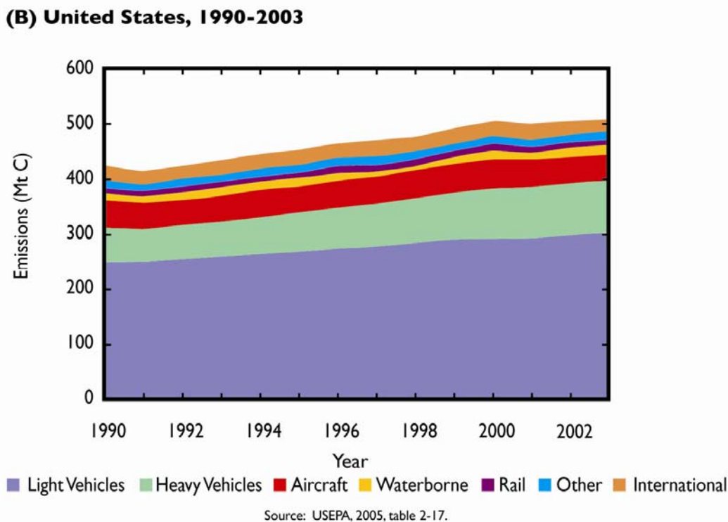
Fig. 7-6B. Transport CO 2 emissions in the United States. Source: U.S. EPA 2005, Table 2-17.
