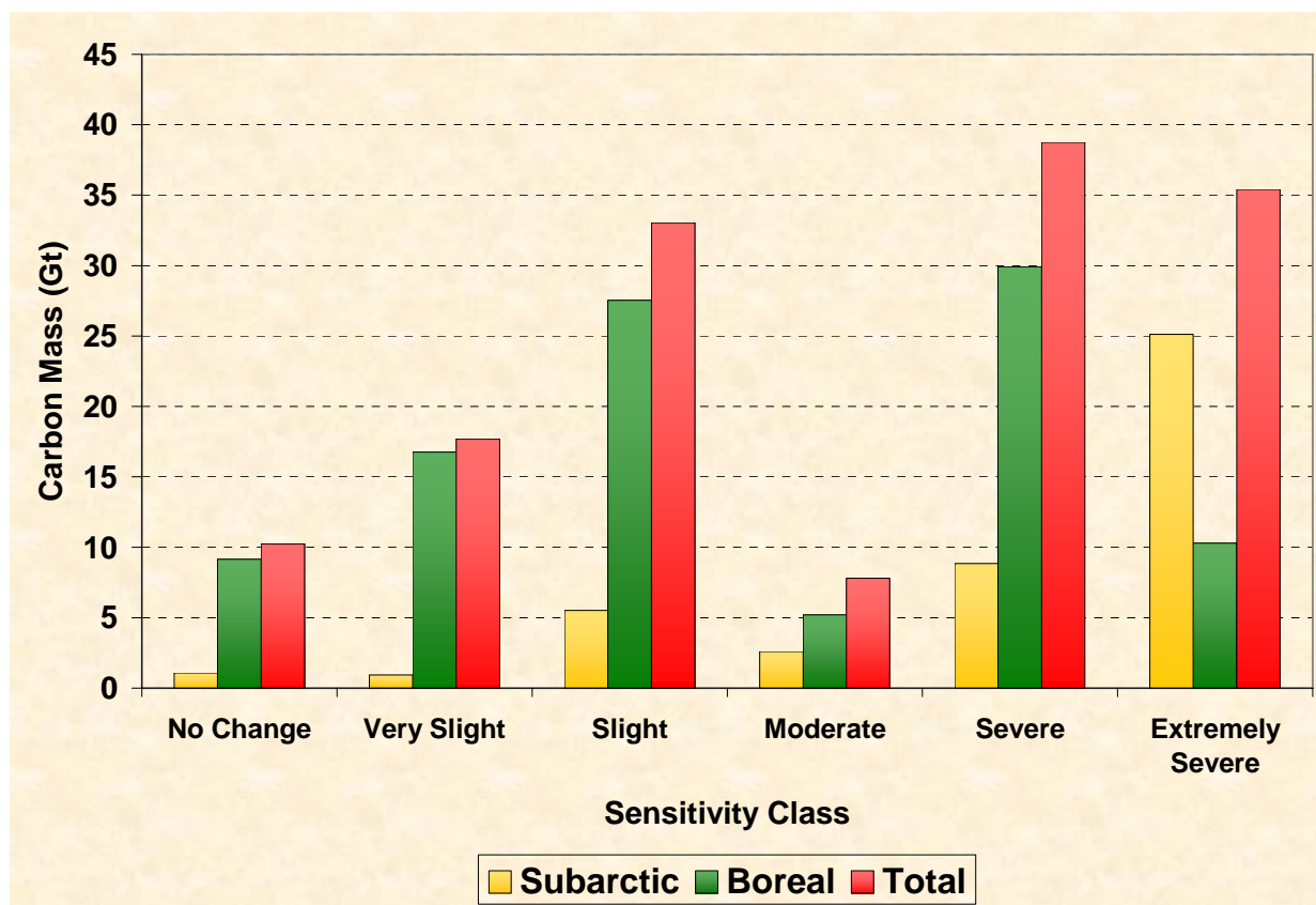
Fig. 12-7. The organic carbon mass in the various sensitivity classes for the Subarctic and Boreal Ecoclimatic Provinces (ecological regions). Source: Tarnocai, 2006.
