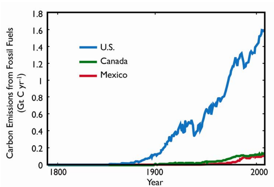
Fig. 3-1. Historical carbon emissions from fossil fuel in the United States, Canada, and Mexico. Data from the U.S. Energy Information Administration (EIA 2005).
