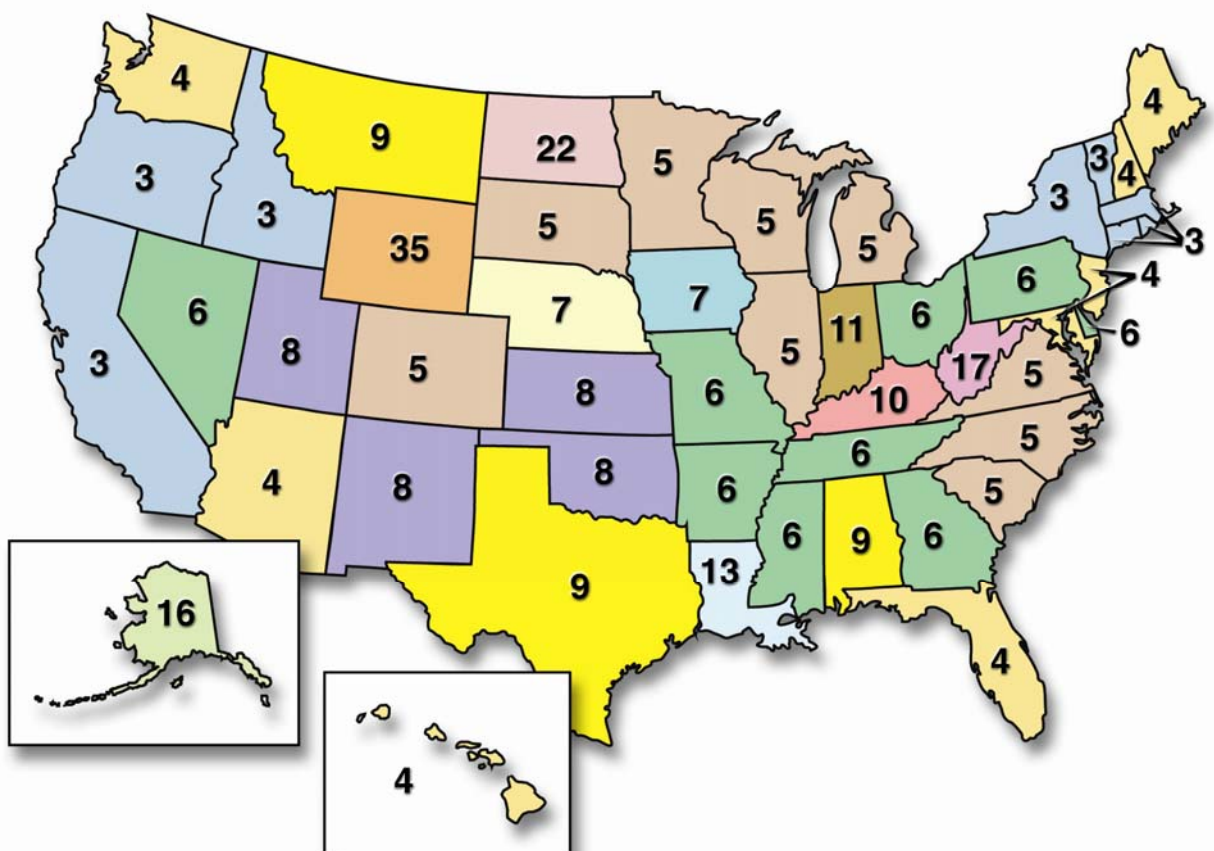
Fig. 9. Per capita emissions of CO 2 from fossil-fuel consumption for the 50 United States in 2000. To demonstrate the range, values have been rounded to whole numbers of metric tons carbon per capita. A large portion of the range for extreme values is related to the occurrence of coal resources and inter-state transfers of electricity. Source: Blasing et al., 2005b.
