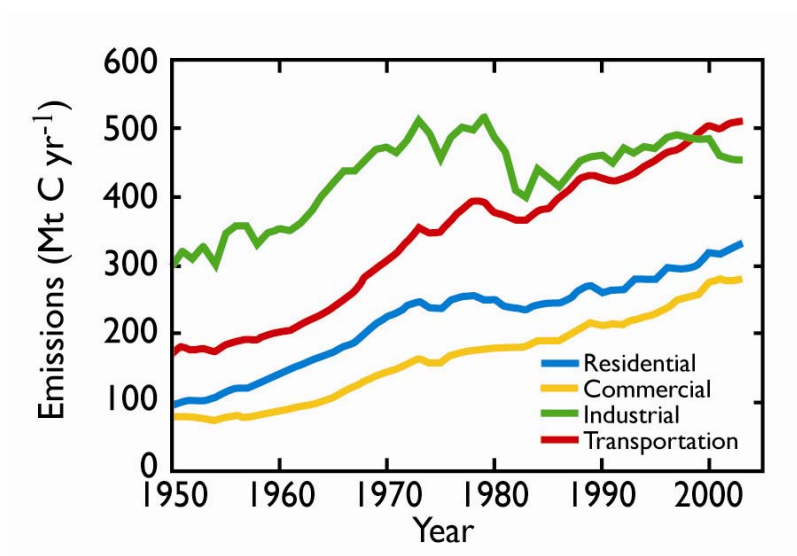
Figure 3-4. Historical U.S. carbon emissions divided among the residential, services, manufacturing, and transportation sectors. Source: EIA (2005).
