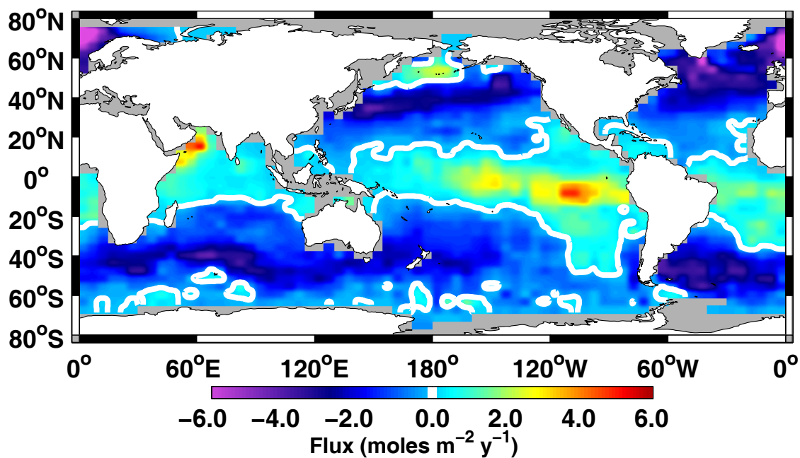
Figure 15-1. Global distribution of sea-air CO 2 flux. The source areas (cyan-green-yellow-orange) are primarily in the tropics with a few high latitude areas where deep mixing occurs in winter. The sink areas (blue-magenta) are located in mid to high latitudes. The white line represents zero flux. Updated from Takahashi et al. (2002).
