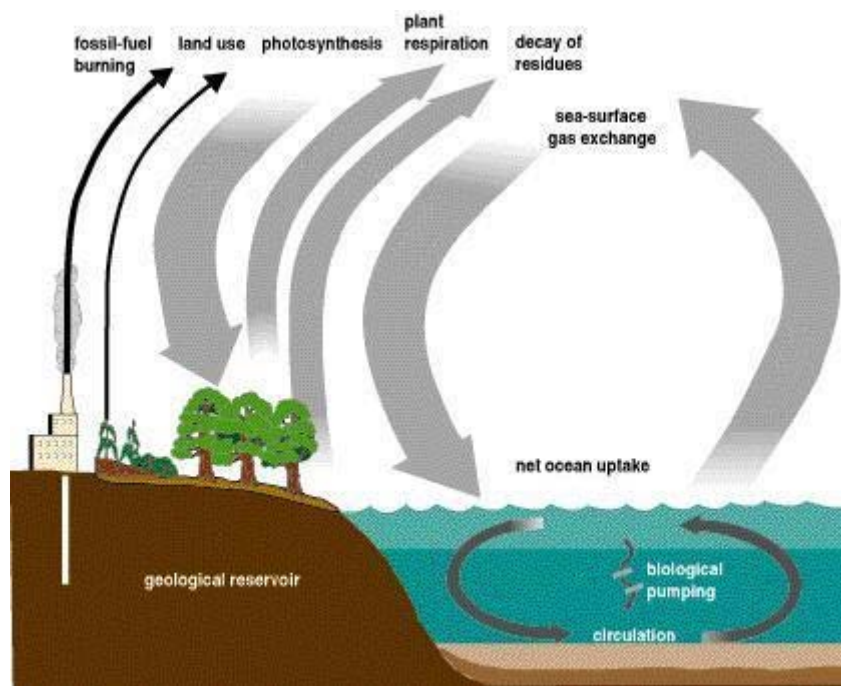
Figure 1-1. The Earth's carbon cycle. Carbon cycles through pools or reservoirs of carbon on land, in the ocean, and in sedimentary rock formations over daily, seasonal, annual, millennial, and geological time scales. See the accompanying text box.
