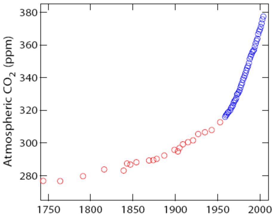
Fig. 2-2. Atmospheric CO 2 concentration from 1750 to 2005. The data prior to 1957 (red circles) are from the Siple ice core (Friedli et al. , 1986). The data since 1957 (blue circles) are from continuous atmospheric sampling at the Mauna Loa Observatory (Hawaii) (Keeling et al. , 1976; Thoning et al. , 1989) (with updates available at http://cdiac.ornl.gov/trends/co2/sio-mlo.htm ).
