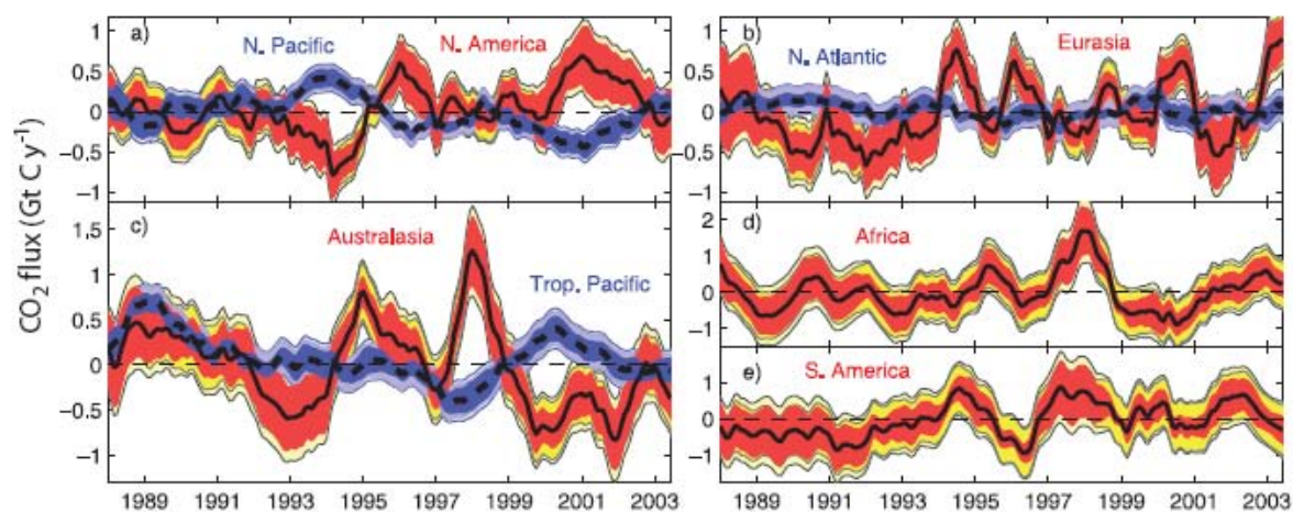
Figure 2-3. The 13-model mean CO 2 flux interannual variability (Gt C per year) for several continents (solid lines) and ocean basins (dashed lines). In each panel, the dark inner band is the 1 \sigma intermodel spread, the lighter adjacent band is the 1 \sigma estimation uncertainty on interannual variability, and the outer band (visible only for the land) is the root sum of squares of the two uncertainty components. (A) North Pacific and North America, (B) Atlantic north of 15°N and Eurasia, (C) Australasia and Tropical Pacific, (D) Africa, and (E) South America (note the different scales for Africa and South America) (Baker et al. , 2006).
