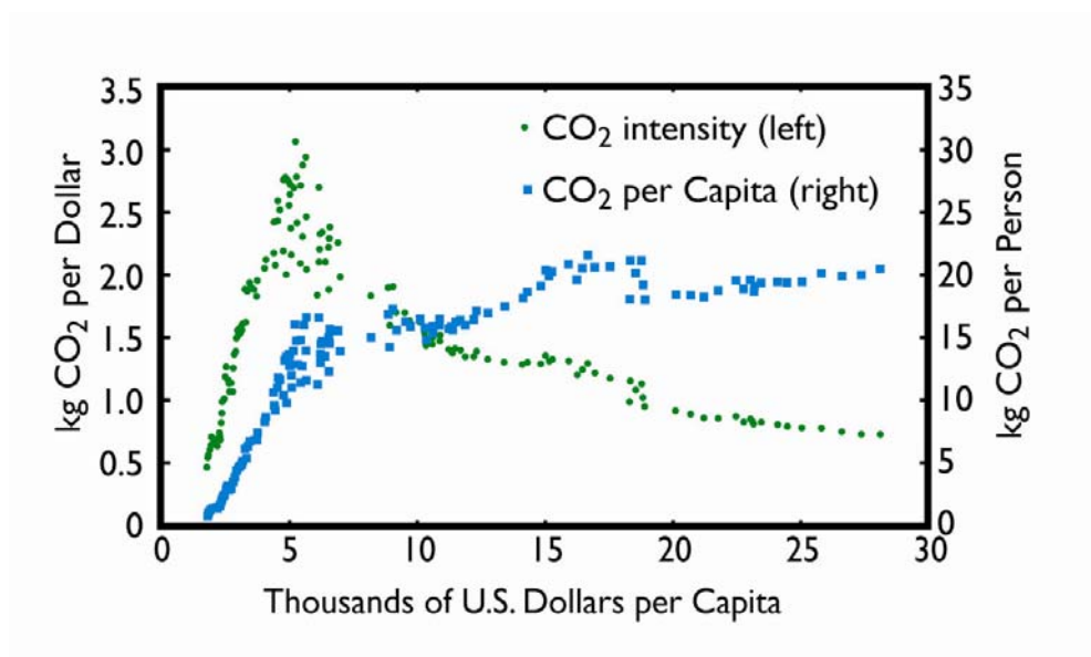
Fig. 3-2. The historical relationship between U.S. per capita GDP and U.S. carbon intensity (green symbols, kg CO 2 emitted per 1995 dollar of GDP) and per capita carbon emissions (blue symbols, kg CO 2 per person). Each symbol shows a different year and each of the two time series progresses roughly chronologically from left (early) to right (late) and ends in 2002. Source: Maddison (2003), Marland et al. (2005). Thus, the red square farthest to the right shows U.S. per capita CO 2 emissions in 2002. The square second farthest to the right shows per capita emissions in 2001. The third farthest to the right shows 2000, and so on. Note that per capita emissions have been roughly constant over the last 30 years (squares corresponding to per capita GDP greater than approximately $16,000).
