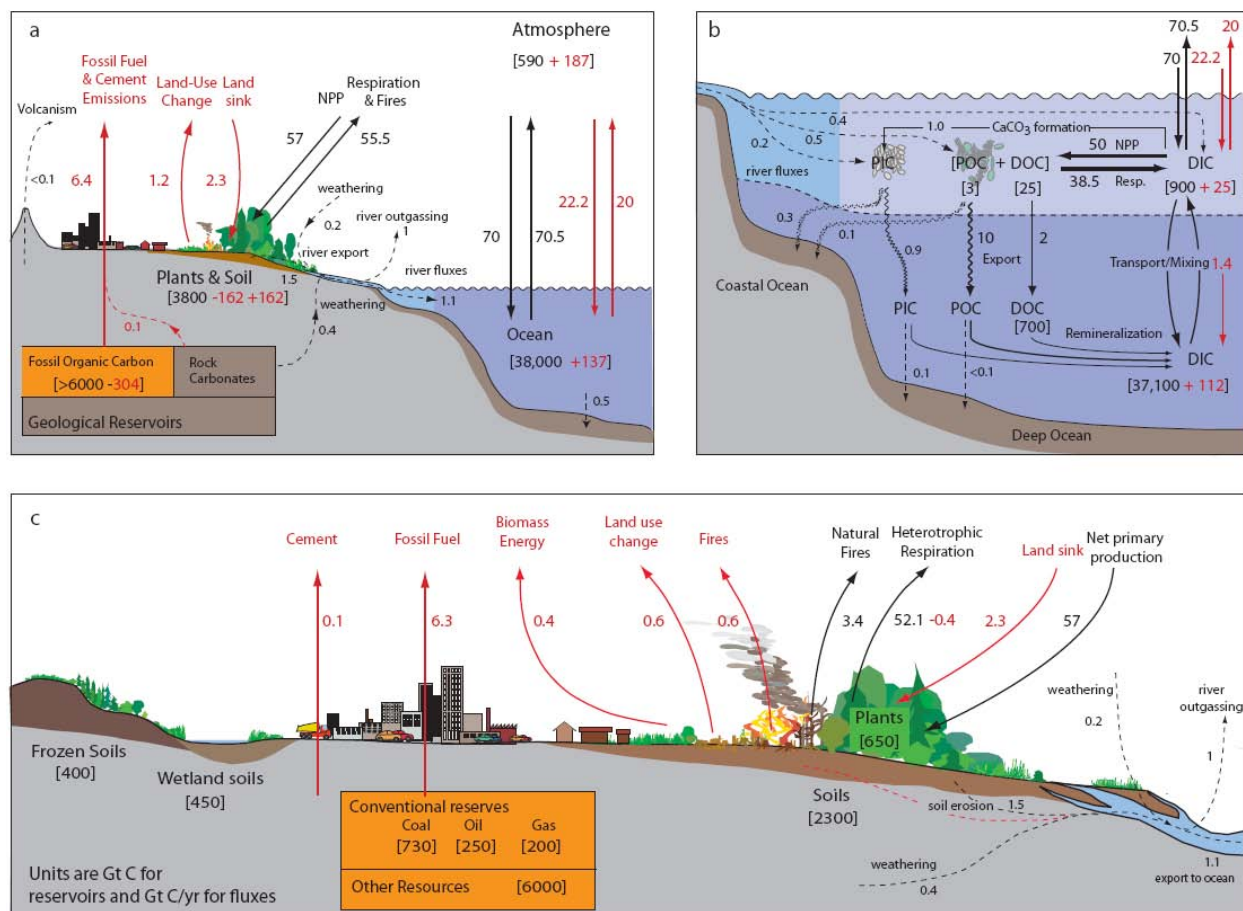
Figure 2-1. Schematic representation of the components of the global carbon cycle. The three panels show (A) the overall cycle, (B) the details of the ocean cycle, and (C) the details of the land cycle. For all panels, carbon stocks are in brackets, and fluxes have no brackets. Stocks and fluxes prior to human-influence are in black. Human-induced perturbations are in red. For stocks, the human-induced perturbations are the cumulative total through 2003. Human-caused fluxes are means for the 1990s (the most recent available data for some fluxes). Redrawn from Sabine et al. (2004b) with updates through 2003 as discussed in the text.
