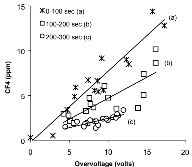
Figure 3: Apparent PFC Emission Rate vs. Cell Overvoltage
