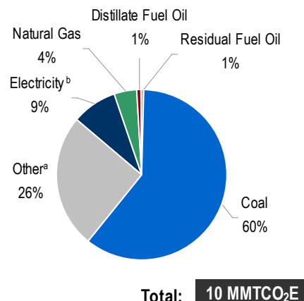
Figure 9-2: 2002 CO 2 Emissions from Energy Consumption in the Lime Sector, by Fuel Type (MMTCO 2 E)
