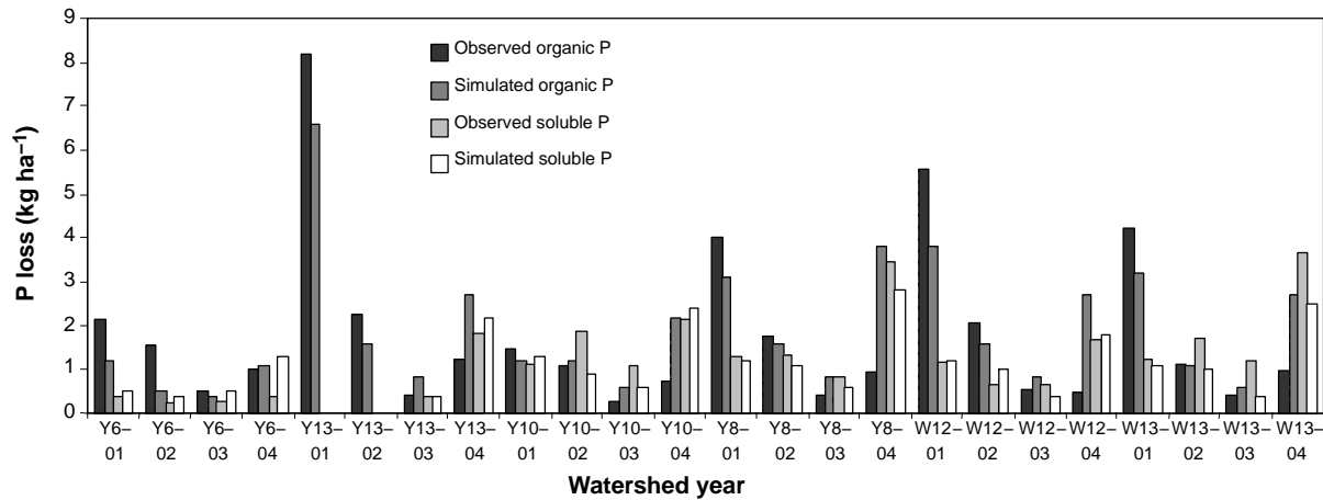
Figure 8. Observed and simulated annual organic P and soluble P losses for the validation period.
