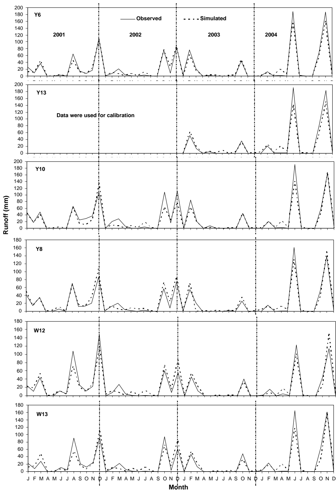
Figure 5. Observed and simulated monthly runoff for the six watersheds for the validation period.
