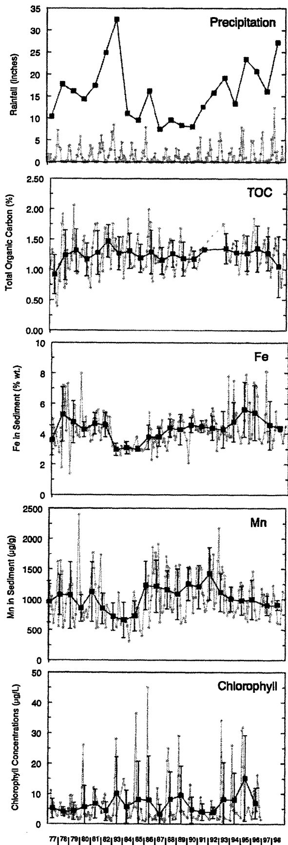
FIGURE 3. Long-term time series trends in precipitation, total organic carbon, Fe (by % wt) and Mn ( \mu\text{g/g} dry weight) in surface sediment, and concentrations ( \mu\text{g/L} ) of chlorophyll (data only available from 1977 to 1996). Monthly data shown in gray; annual means shown in black.
