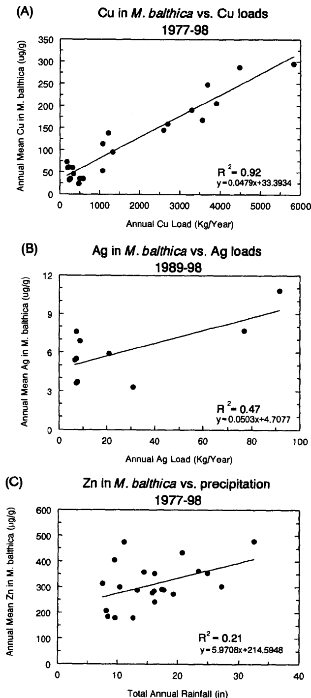
FIGURE 5. (A) Annual average Cu concentration in M. balthica ( \mu\text{g/g} dry weight) vs total annual Cu load (kg/yr). (B) Annual average Ag concentration in M. balthica ( \mu\text{g/g} dry weight) vs total annual Ag load (kg/yr). (C) Annual average Zn concentration in M. balthica ( \mu\text{g/g} dry weight) vs annual precipitation (in).
