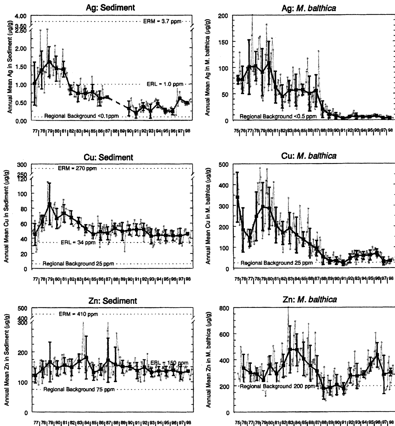
FIGURE 4. Annual trends of Ag, Cu, and Zn surface sediments (1977–1998) and M. balthica (1975–1998) from the Palo Alto mudflat. All concentrations are reported in \mu\text{g/g} dry weight. Regional background (4) and ERL and ERM values (29) are indicated for each element by the dashed line.
