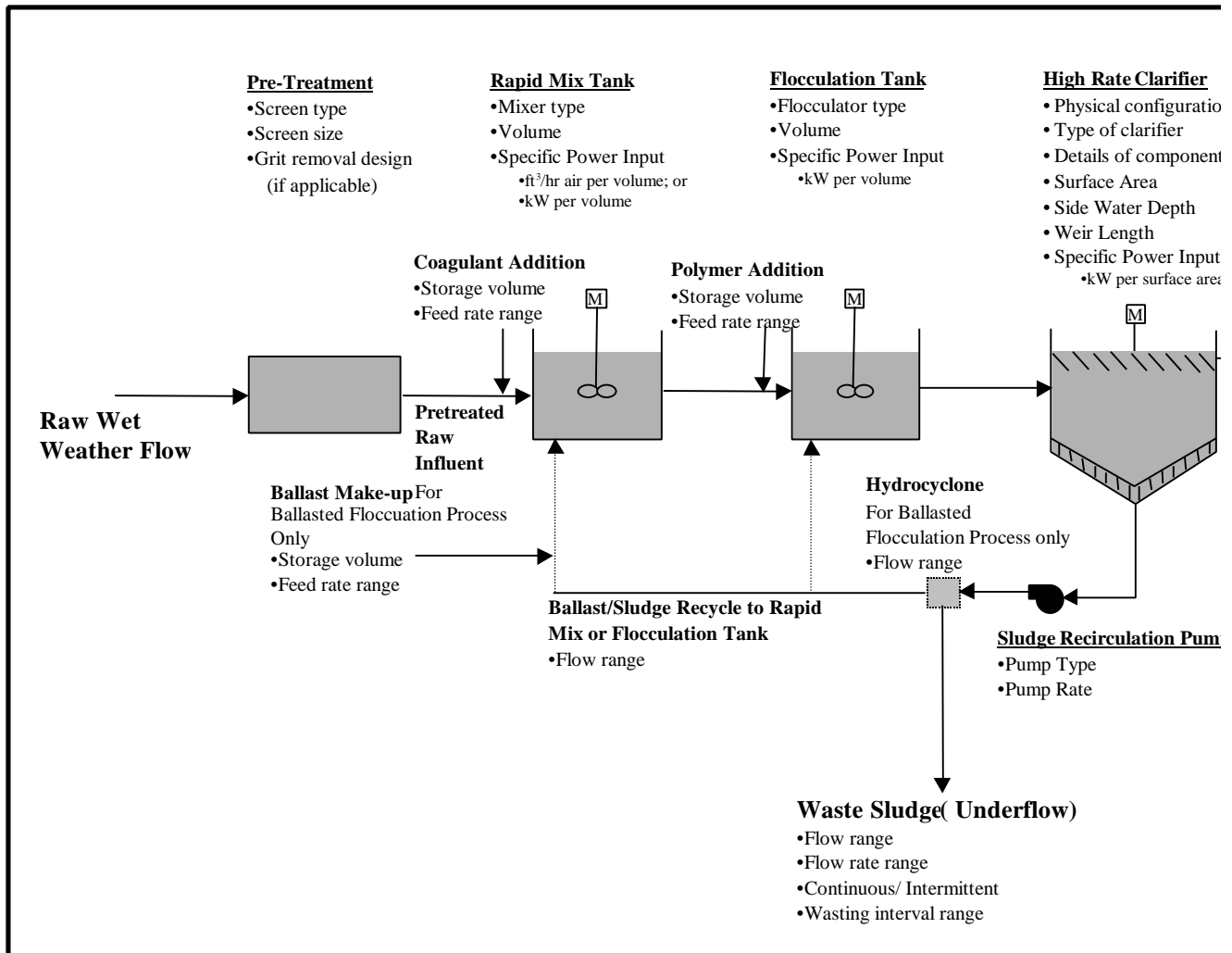
Figure 2.1 Schematic of a Typical Chemically-Enhanced High-Rate Separation
