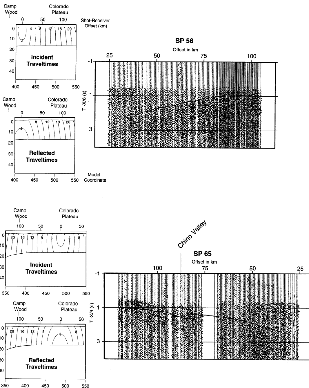
Figure 8. Partial shot records from shots 56 and 65 windowed to highlight the middle crustal reflections. Calculated travel times are shown on the data. The kink in the reflection from shot 65 is a delay from Chino Valley, a sedimentary basin adjacent to the physiographic edge of the Colorado Plateau (not seen on shot 56 because it was located \sim 5 km north of Chino Valley).
