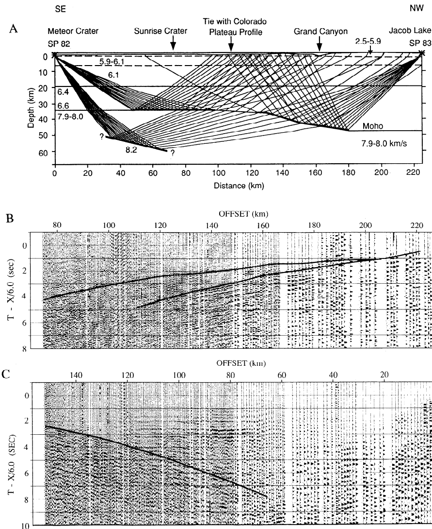
Figure 11. (a) Velocity model derived from the PACE 1989 Grand Canyon profile and data plots for shots (b) 82 and (c) 83. Ray coverage for the Moho and the upper mantle interface is shown in Figure 11a, and the corresponding calculated travel time curves are plotted in Figures 11b and 11c. Midpoint coverage is shown by the heavy black lines. Earlier PmP arrivals from the southeast off-end shot (82) suggest a thinner crust on the southeast end of the profile where it ties to the Colorado Plateau line. Later arrivals from the northwest shot (83) suggest a thicker crust to the north. The data were plotted with a low-frequency (0–7 Hz) band-pass filter. Details on the model are discussed in the text.
