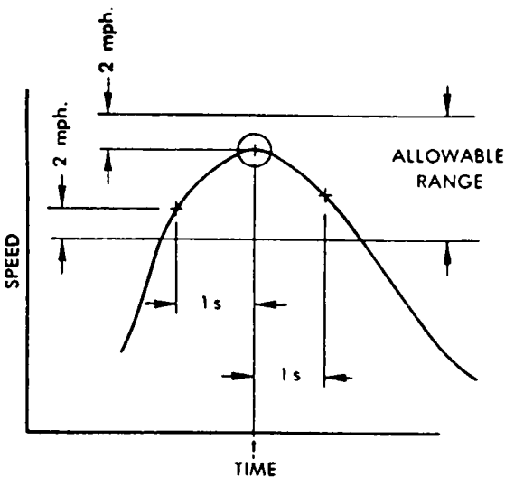
FIGURE B78-4b—DRIVERS TRACE, ALLOWABLE RANGE
