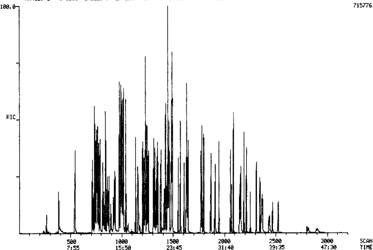
FIGURE 6 Chromatogram of Combined Acid/base/neutral Standard.
