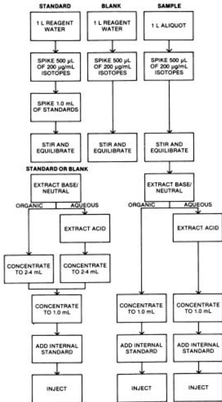
FIGURE 4 Flow Chart for Extraction/Concentration of Precision and Recovery Standard, Blank, and Sample by Method 1625. Numbers in Brackets [ ] Refer to Section Numbers in the Method.
