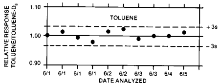
FIGURE 7 Quality Control Charts Showing Area (top graph) and Relative Response of Toluene to Toluene- d_8 (lower graph) Plotted as a Function of Time or Analysis Number.
