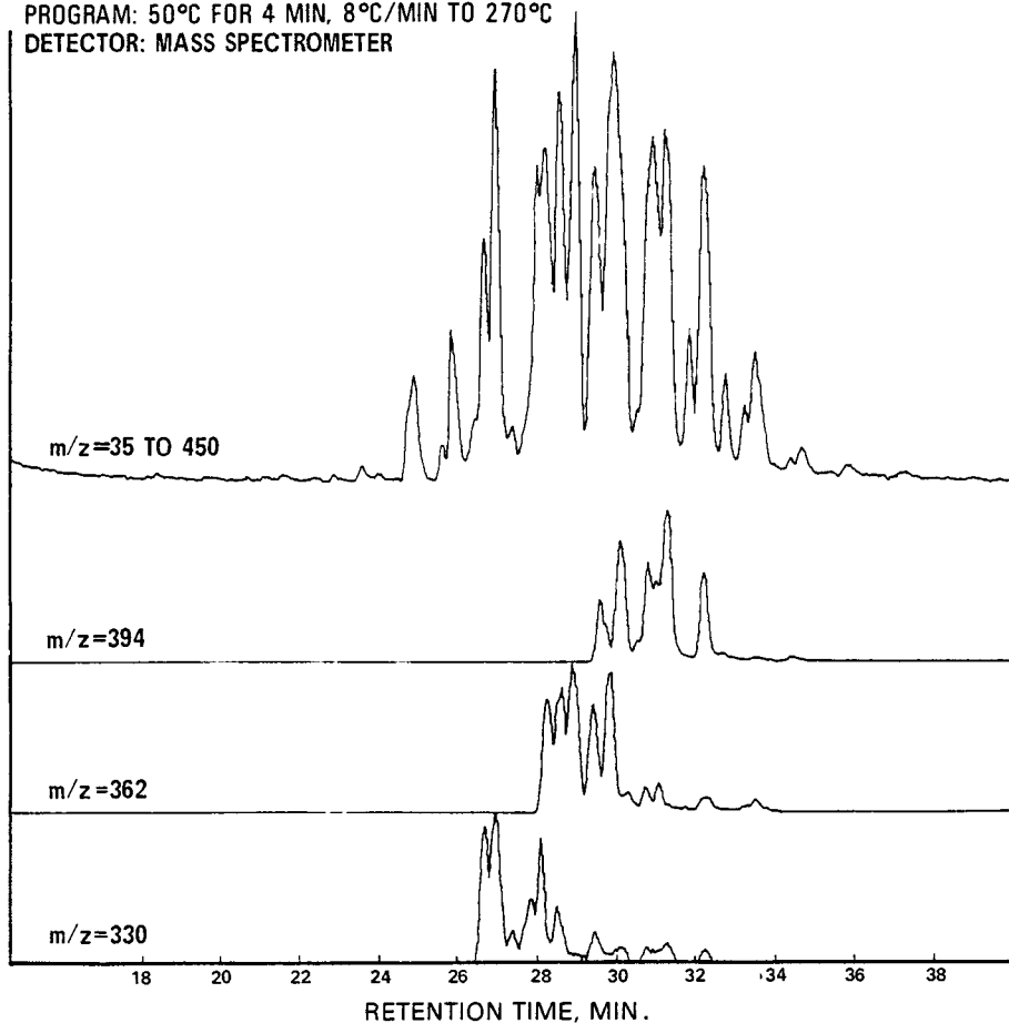
Figure 12. Gas chromatogram of PCB-1260.
