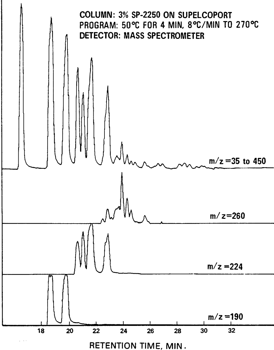
Figure 7. Gas chromatogram of PCB-1221.
