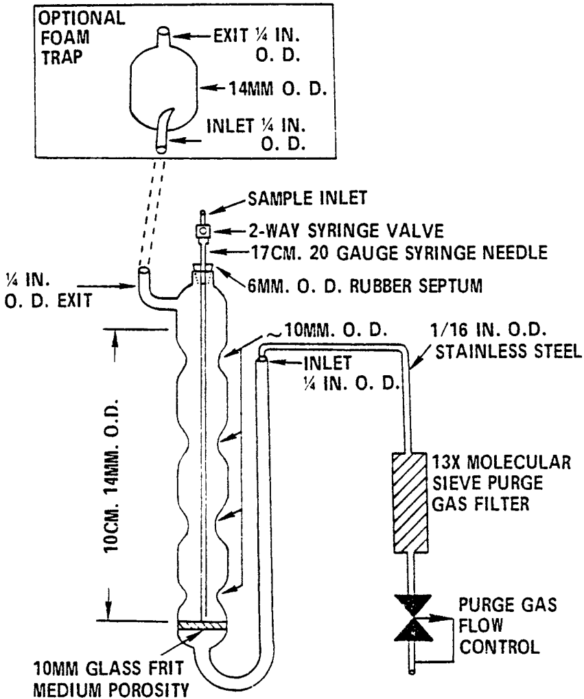
Figure 1. Purging device.
