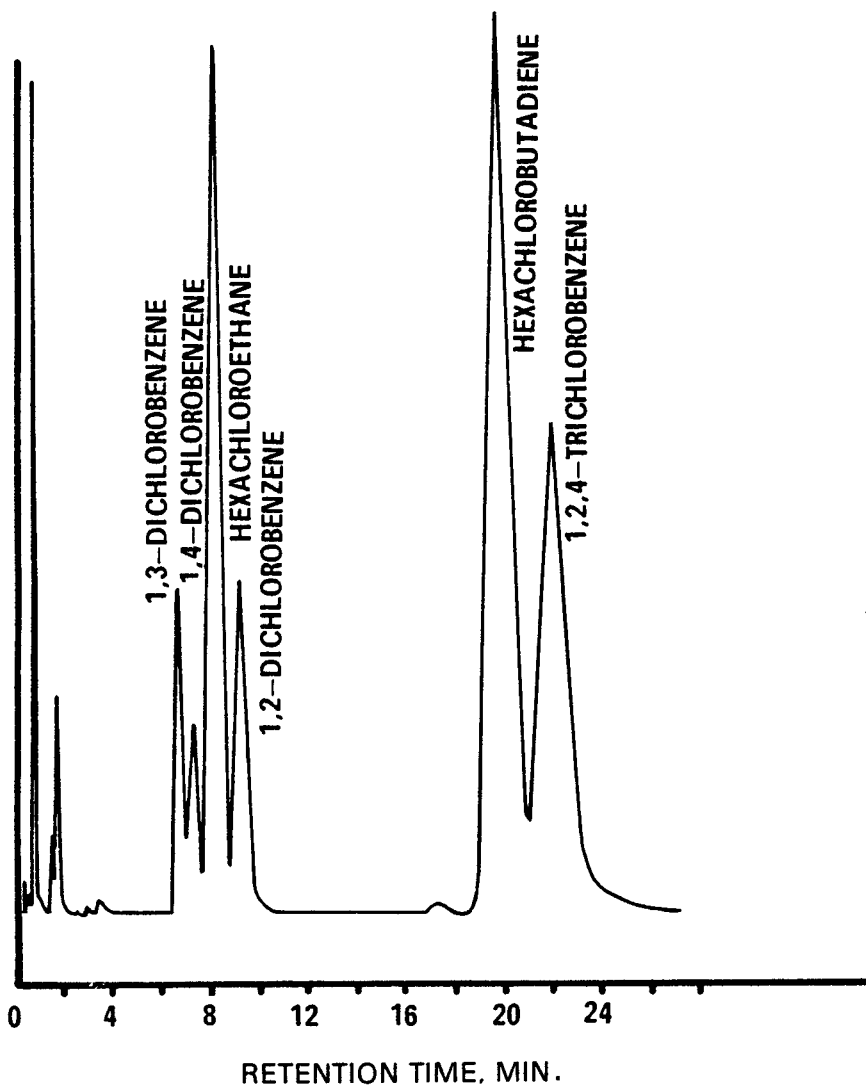
Figure 1. Gas chromatogram of chlorinated hydrocarbons.
