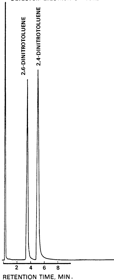
Figure 2. Gas chromatogram of dinitrotoluenes.
