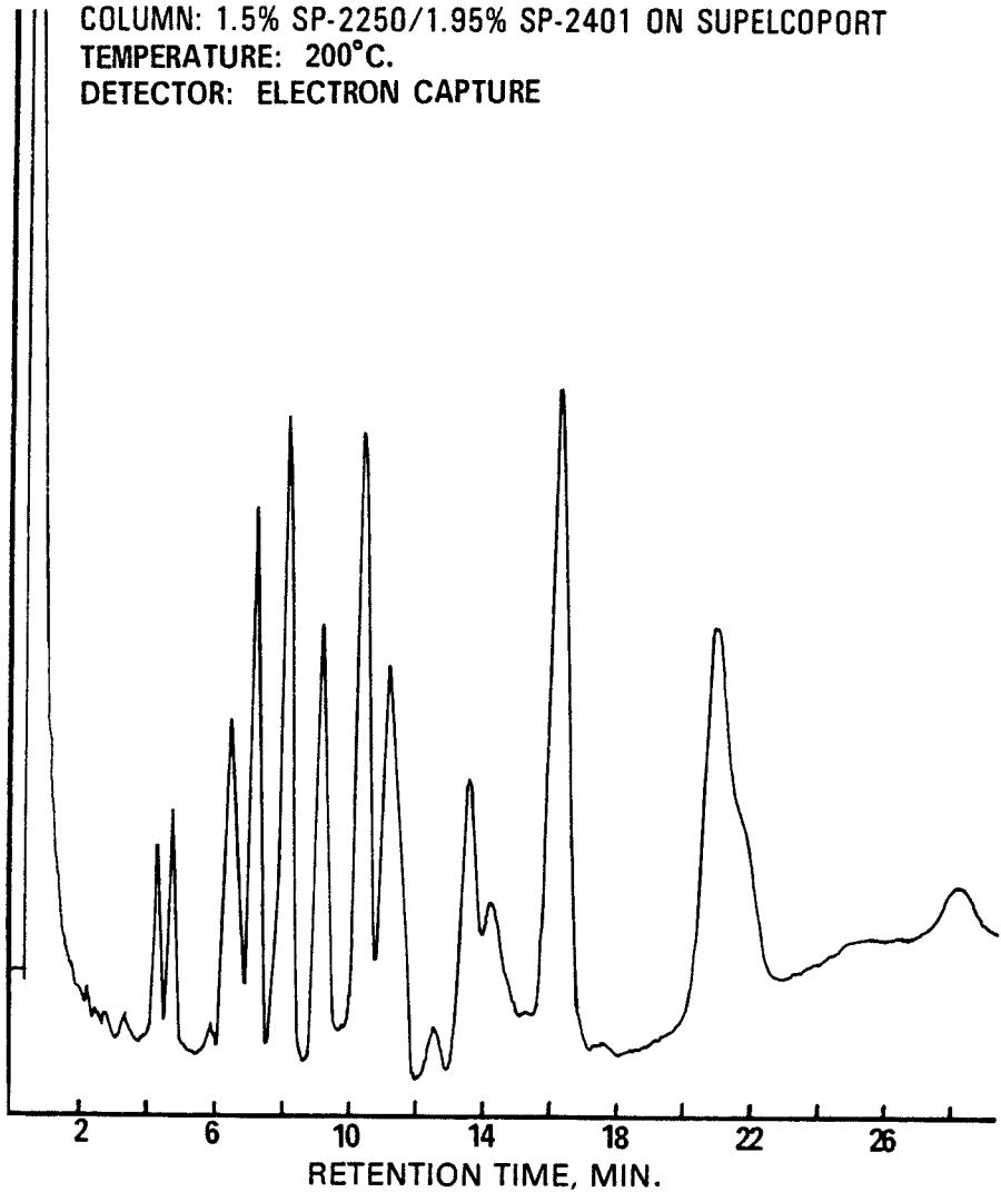
Figure 10. Gas chromatogram of PCB-1260.
