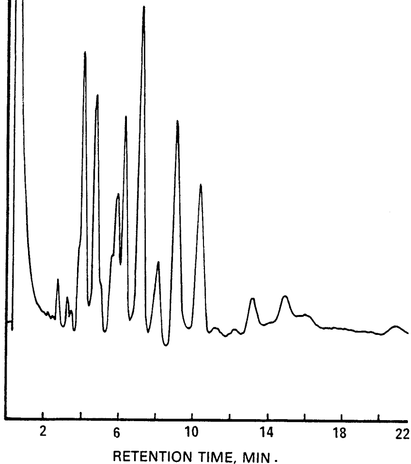
Figure 9. Gas chromatogram of PCB-1254.
