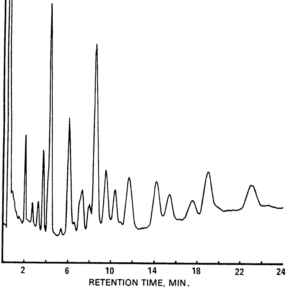
Figure 6. Gas chromatogram of PCB-1232.
