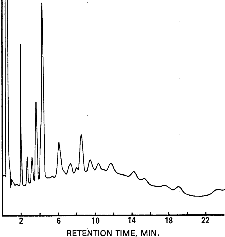
Figure 5. Gas chromatogram of PCB-1221.
