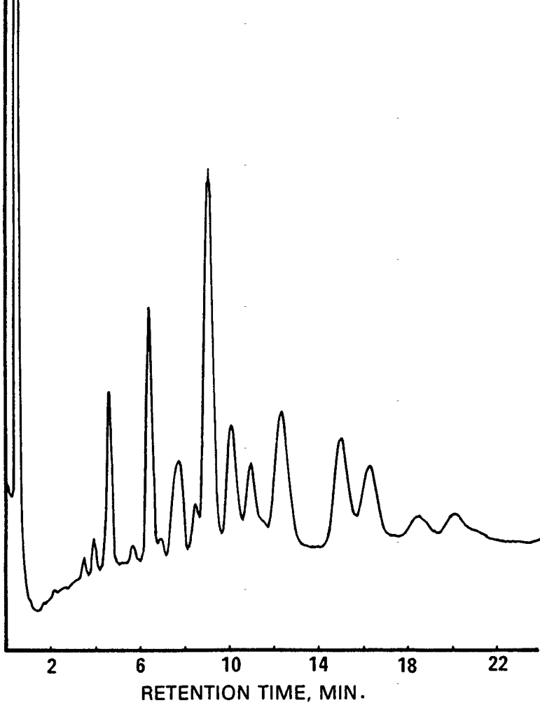
Figure 4. Gas chromatogram of PCB-1016.
