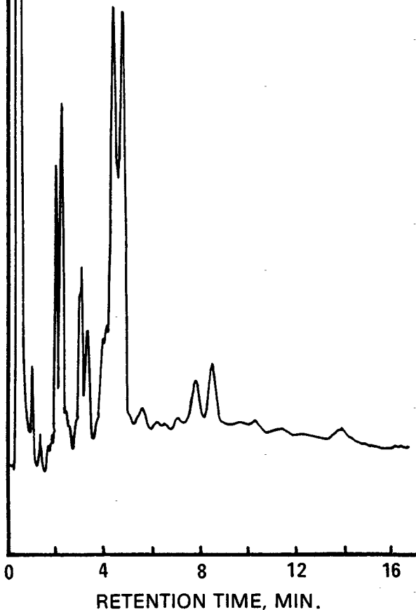
Figure 2. Gas chromatogram of chlordane.
