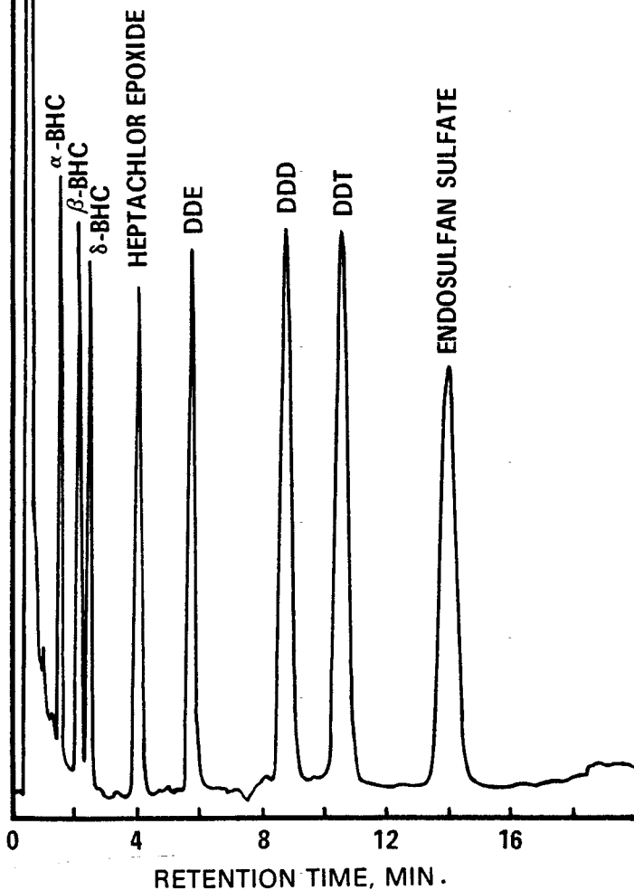
Figure 1. Gas chromatogram of pesticides.
