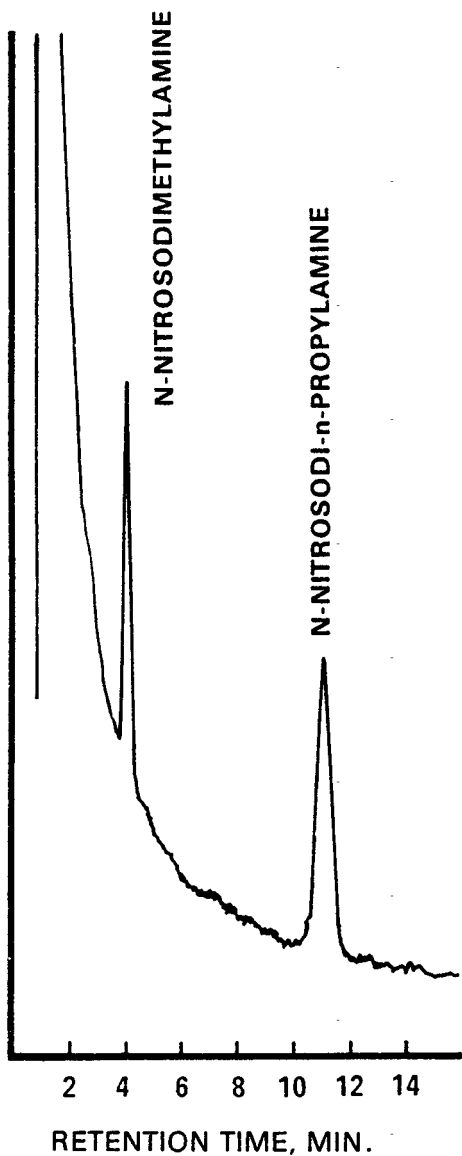
Figure 1. Gas chromatogram of nitrosamines.
