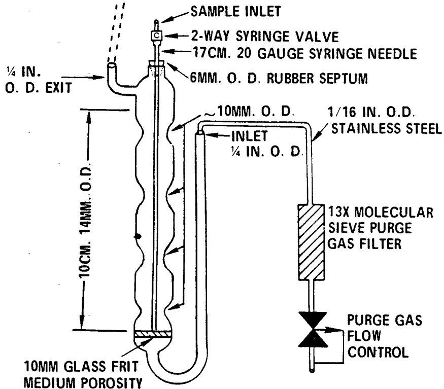
Figure 1. Purging device.
