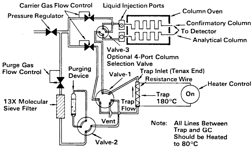
Figure 5. Purge and trap system-desorb mode.
