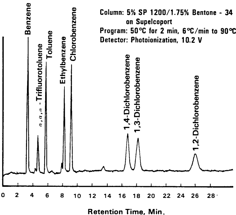
Figure 6. Gas chromatogram of purgeable aromatics.
