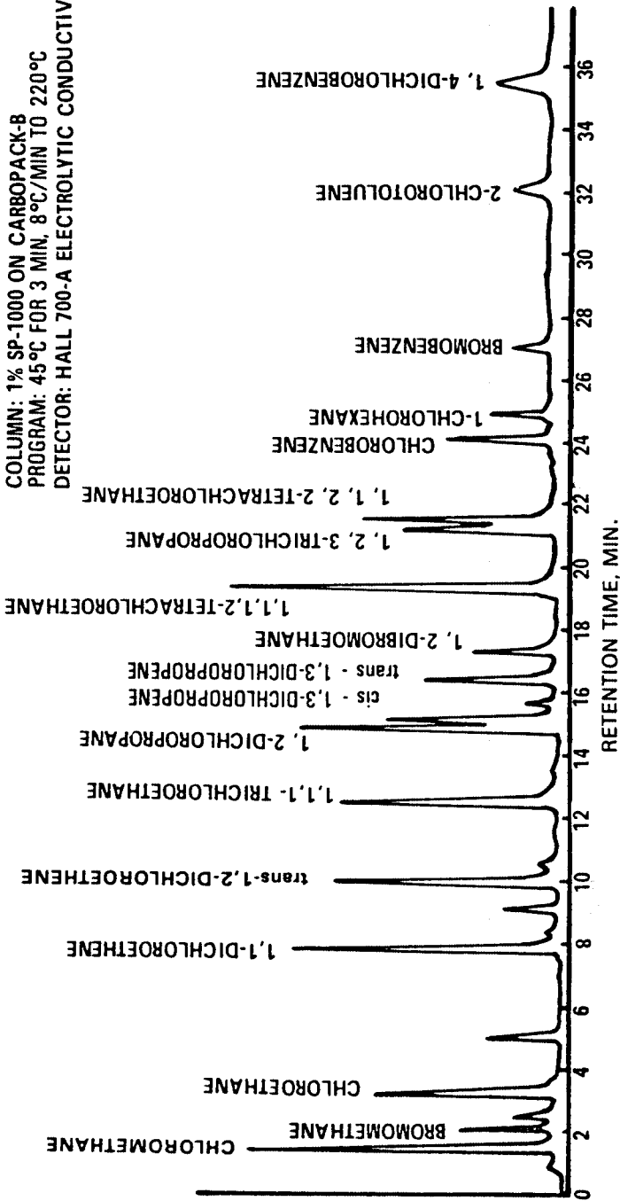
Figure 5. Gas chromatogram of purgable halocarbons.
