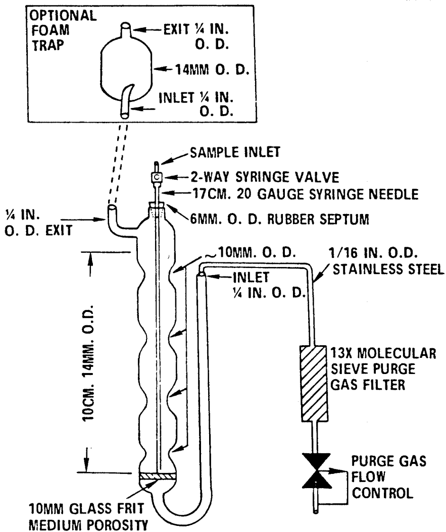
Figure 1. Purging device.
