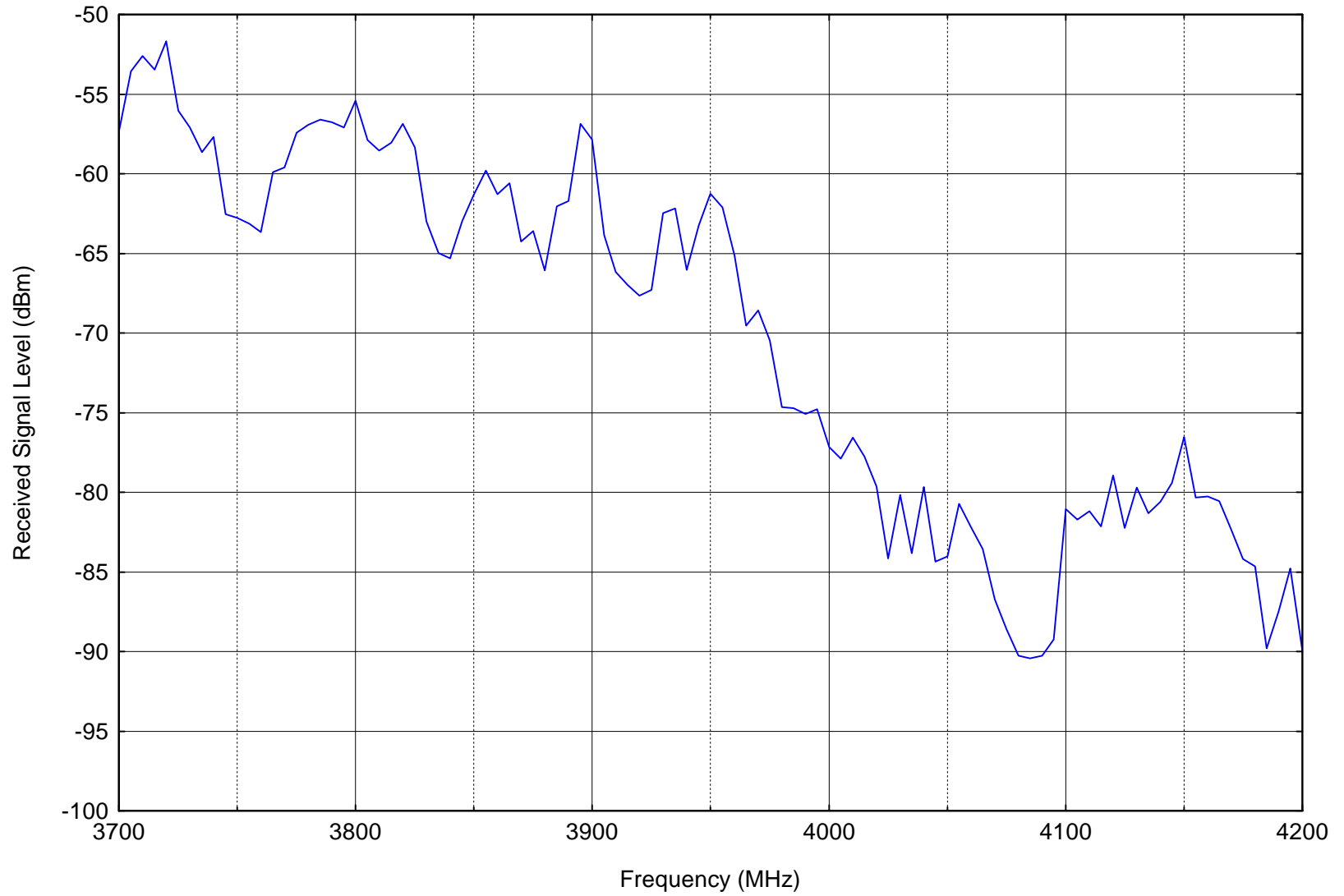
Figure 16. Radar emission spectrum measured in south parking lot
