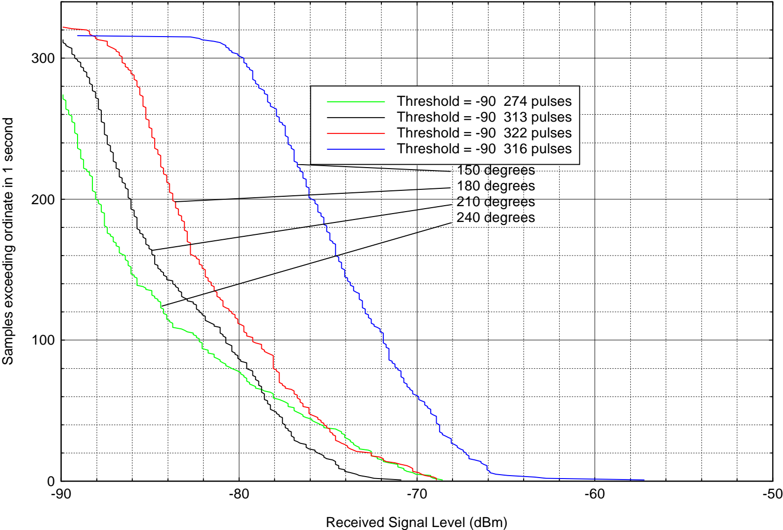
Figure 14. APDs for south parking lot, 150-240 degrees azimuth
