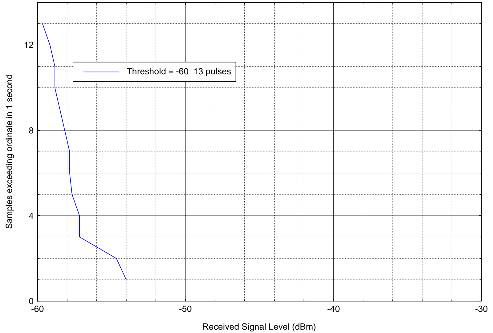
Figure 8. Interference threshold APD; radar=low power, pier 3, bands 8-10
