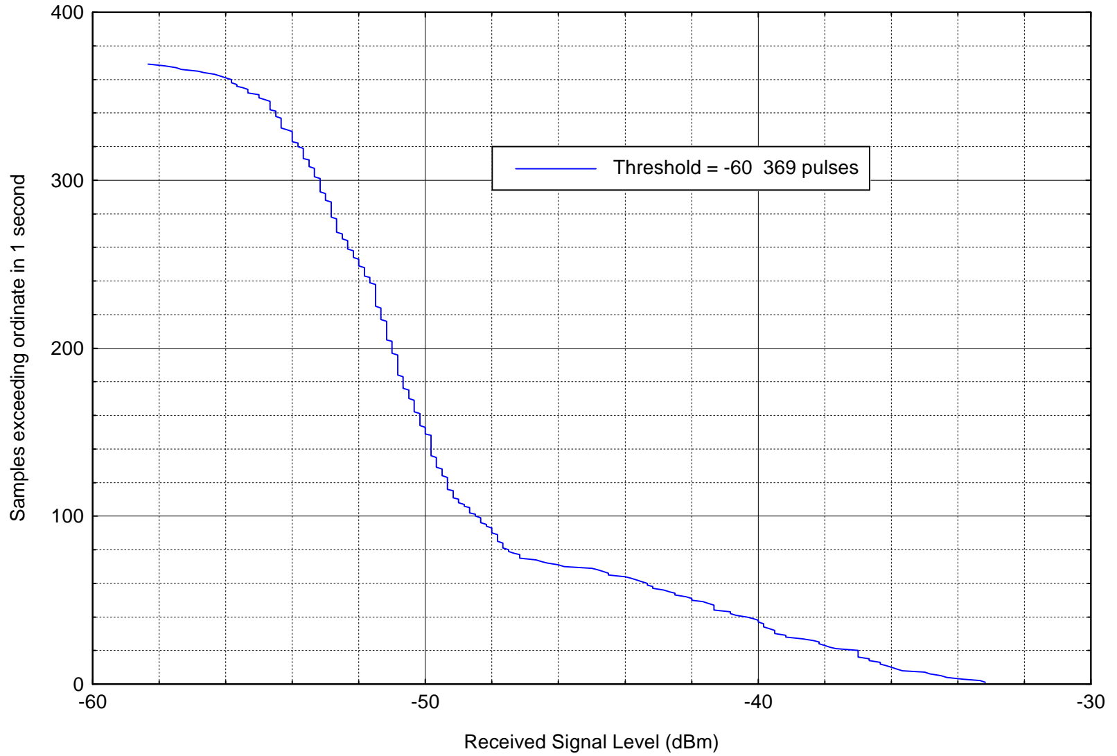
Figure 7. Receiver worst-case APD; radar = high power, pier 3, bands 8-10
