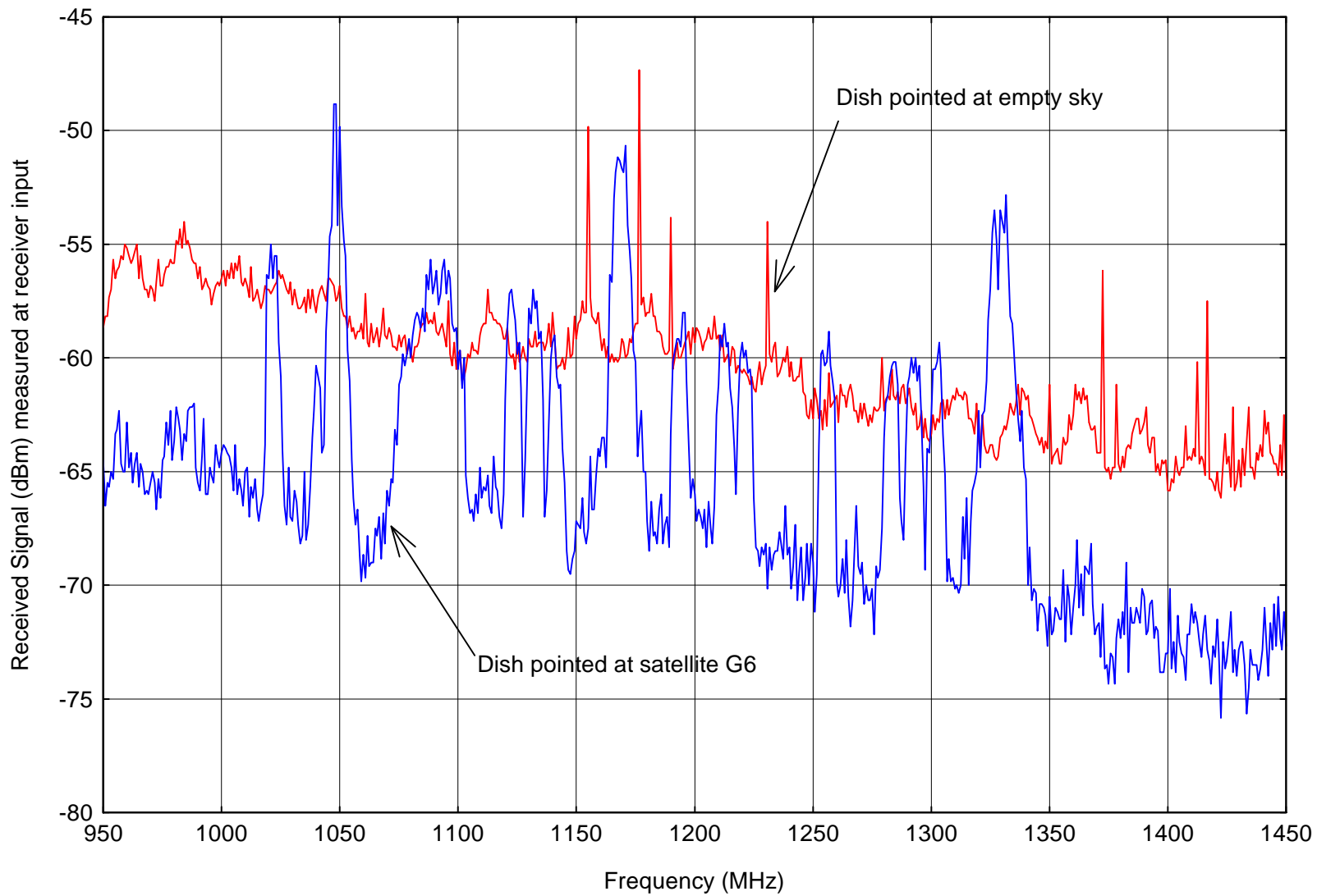
Figure 6. LNB noise floor with transponder signals vs. noise floor with LNB terd
