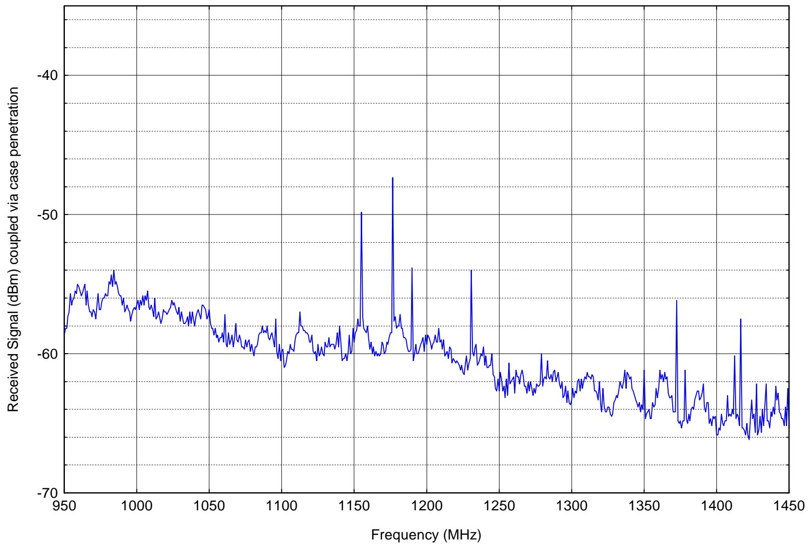
Figure 4. Earth station w. 50-ohm load, no bandpass filter, radar coupling
