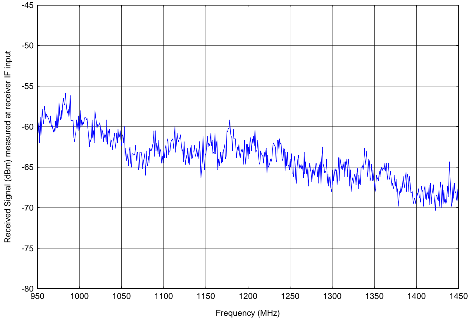
Figure 2. Earth station antenna pivoted away from satellite; LNB noise only
