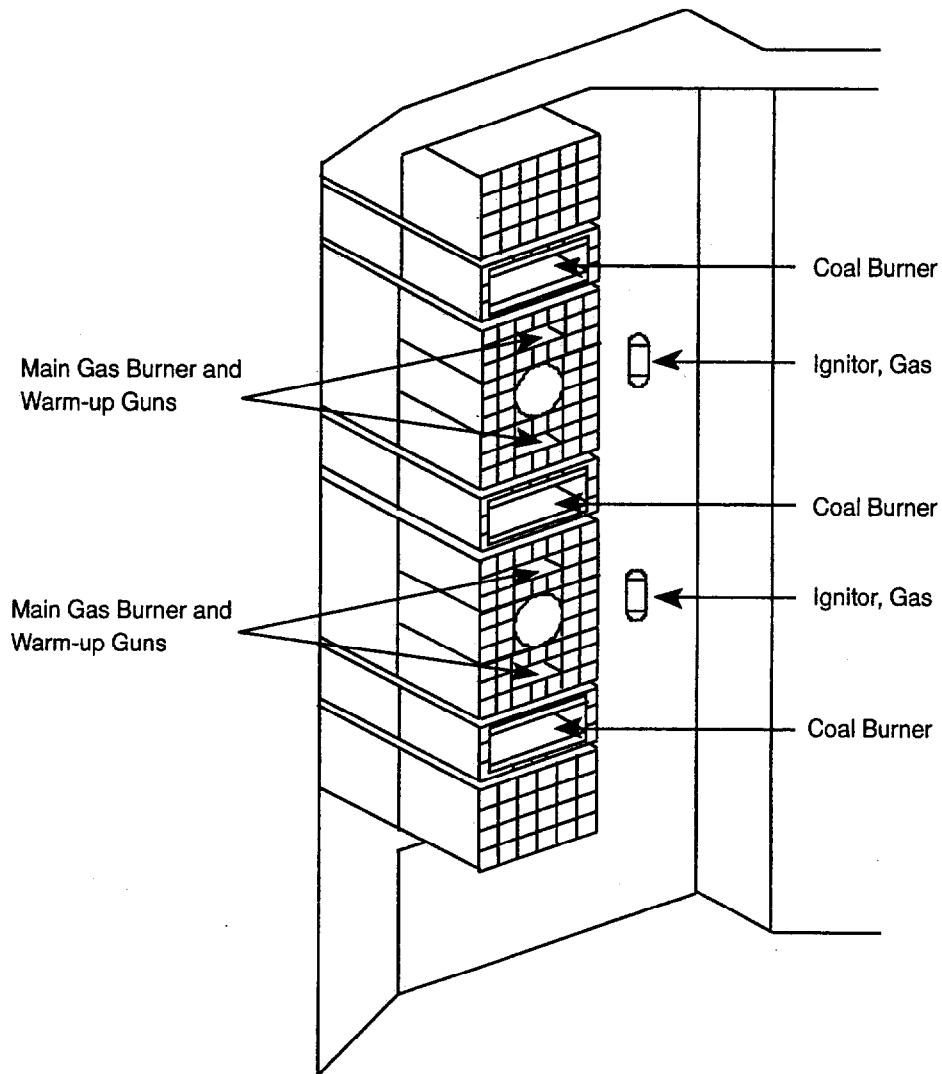
Figure 3-8. Hennepin Unit 1—Stacked Burners of Tangentially-Fired Boiler (Angello et al., 1992).
