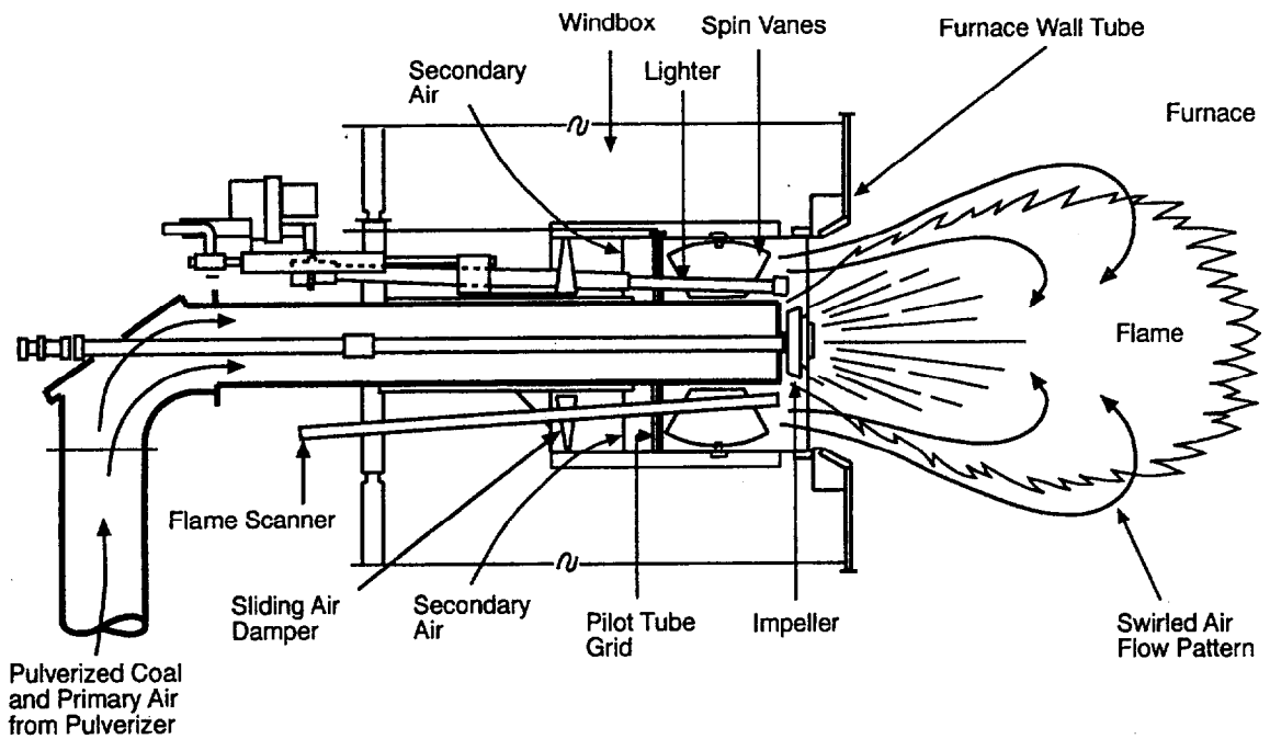
Figure 2-9. Typical Circular Burner (Stultz and Kitto, 1992).
