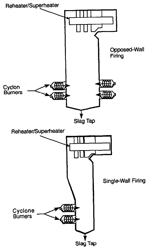
Figure 2-13. Firing Arrangements Used with Cyclone-Fired Boilers (Stultz and Kitto, 1992).
