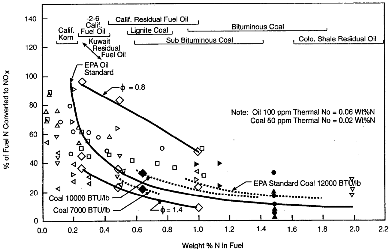
Figure 2-3. Conversion of Fuel-Bound Nitrogen in Practical Combustors (Pohl and Sarofim, 1976).
