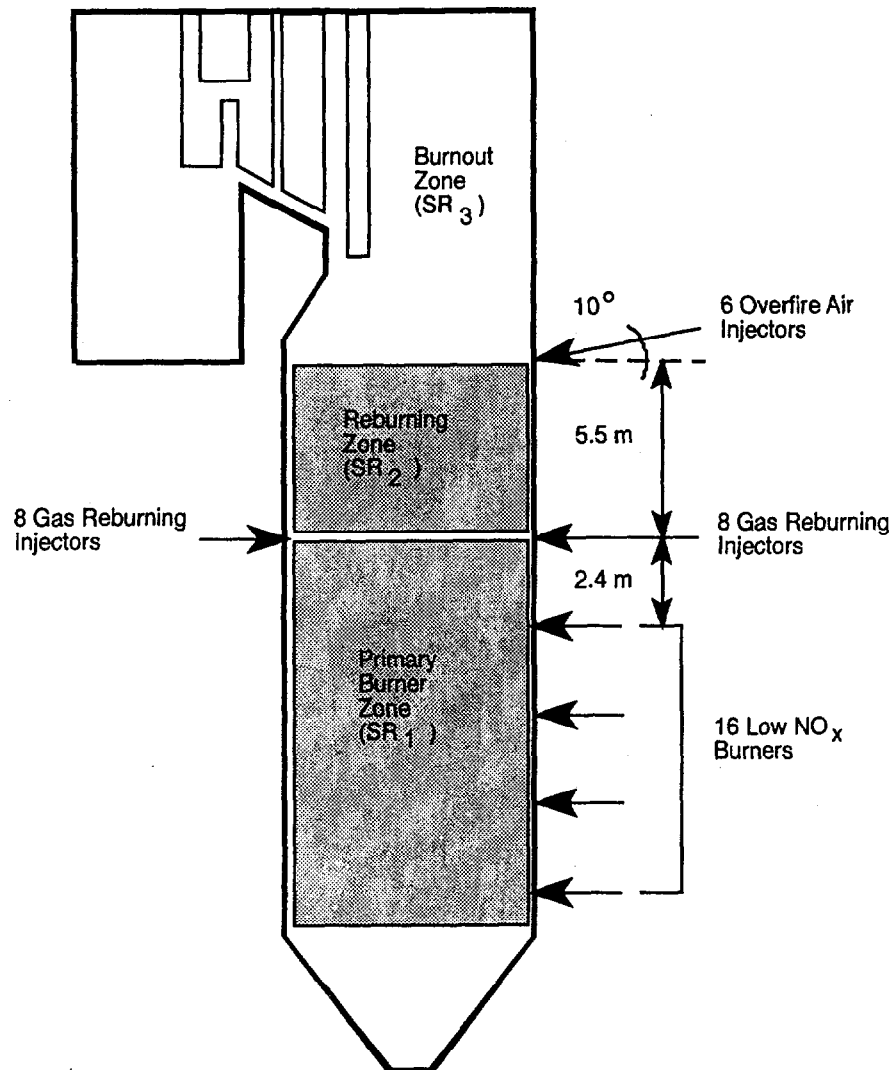
Figure 3-1. Cherokee Unit 3-LNB-Gas Reburn System Schematic (Sanyal et al., 1993).
