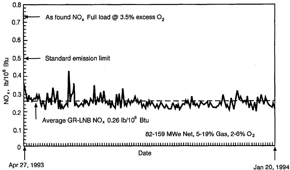
Figure 3-7. Cherokee Unit 3—Long-Term NO x Emission Data (Sanyal et al., 1993).
