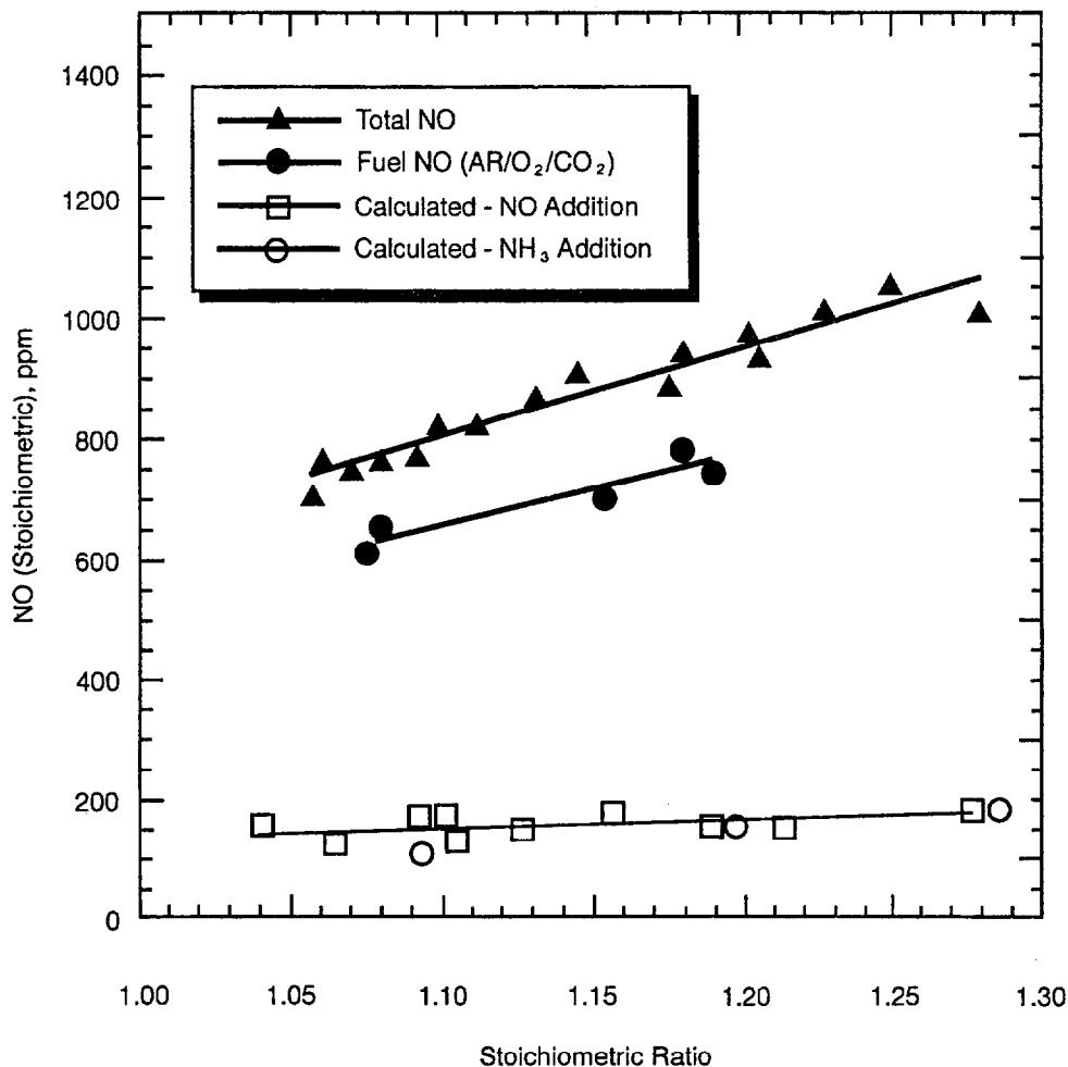
Figure 2-4. Sources of NO x Emissions from Coal (Pershing and Wendt, 1976).
