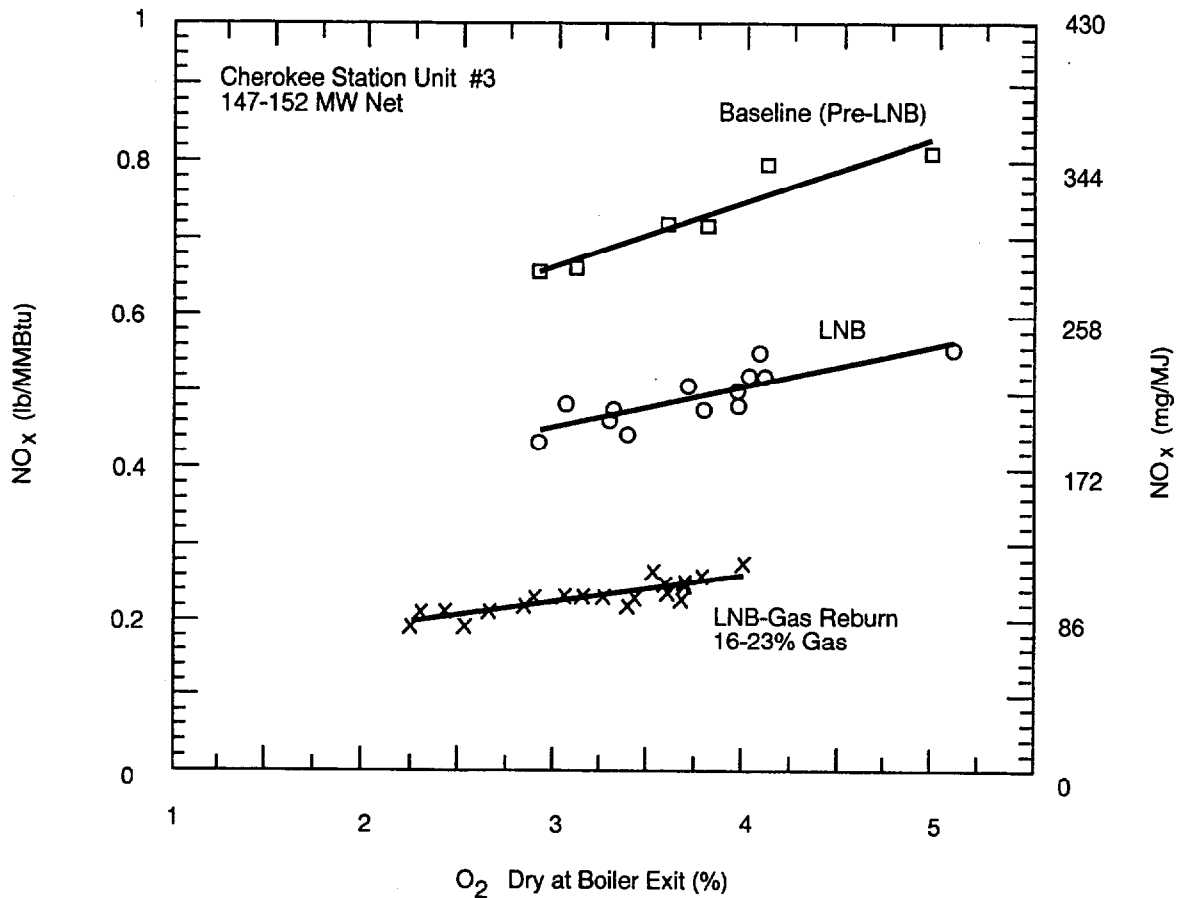
Figure 3-4. Cherokee Unit 3—Effect of Excess Air on NO x Emissions (Sanyal et al., 1993).
