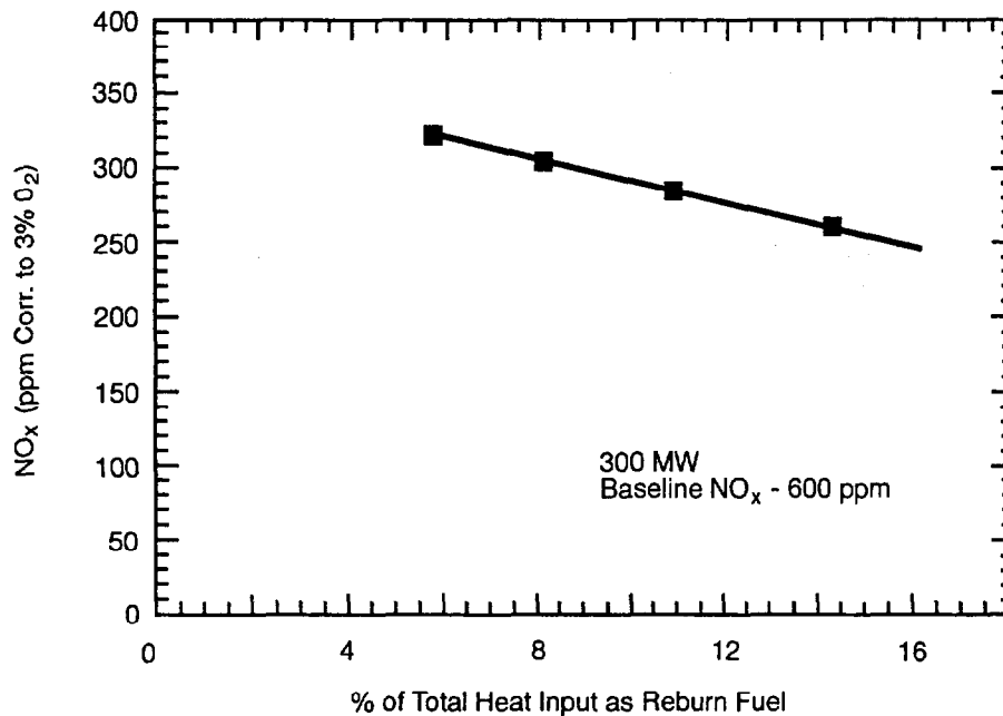
Figure 3-23. Ladyzhin Unit 4-NO x Emissions vs. Reburn Fuel Percentage (LaFlesh et al., 1993).
