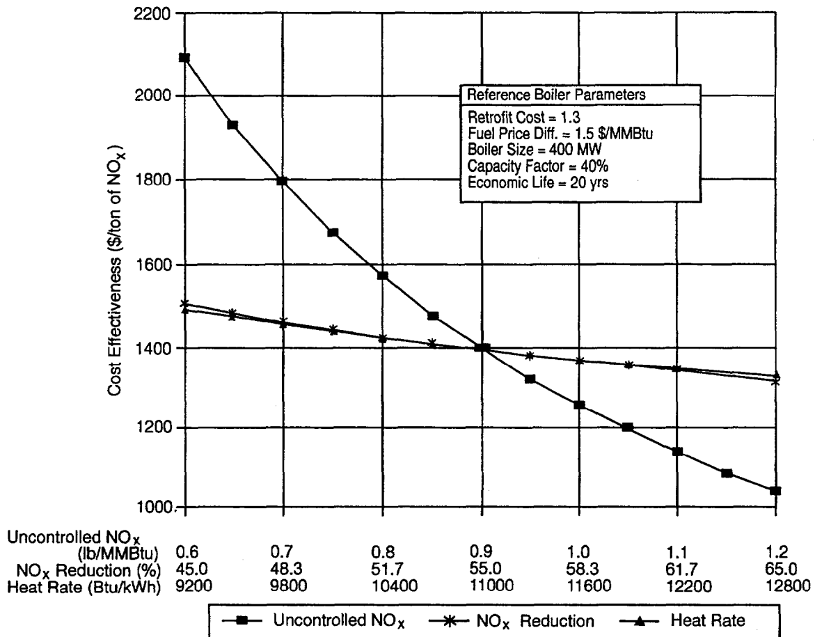
Figure 4-2. Impact of NO x Emission Characteristics and Heat Rate on Reburn Cost Effectiveness for Wall-Fired Boilers (U.S. EPA, 1994).
