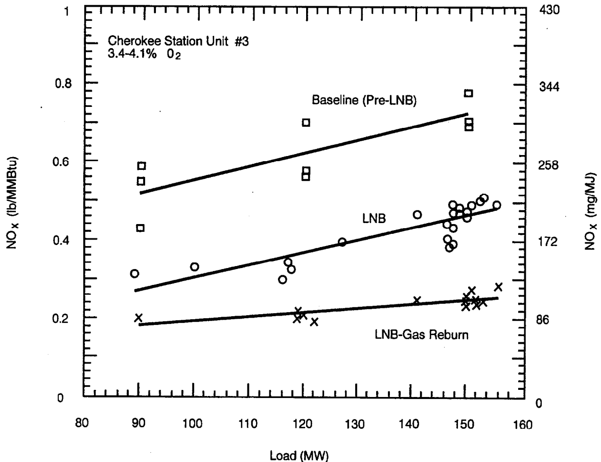
Figure 3-6. Cherokee Unit 3—Effect of Unit Load on NO x Emissions (Sanyal et al., 1993).
