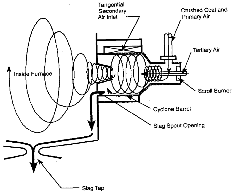
Figure 2-12. Cyclone Burner (Farzan, et al., 1991).
