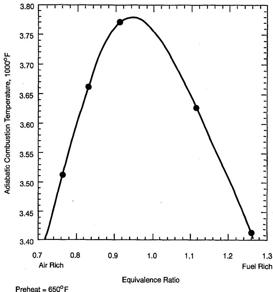
Figure 2-2. Effect of Equivalence Ratio on Adiabatic Combustion Temperature (Bagwell et al., 1971).
