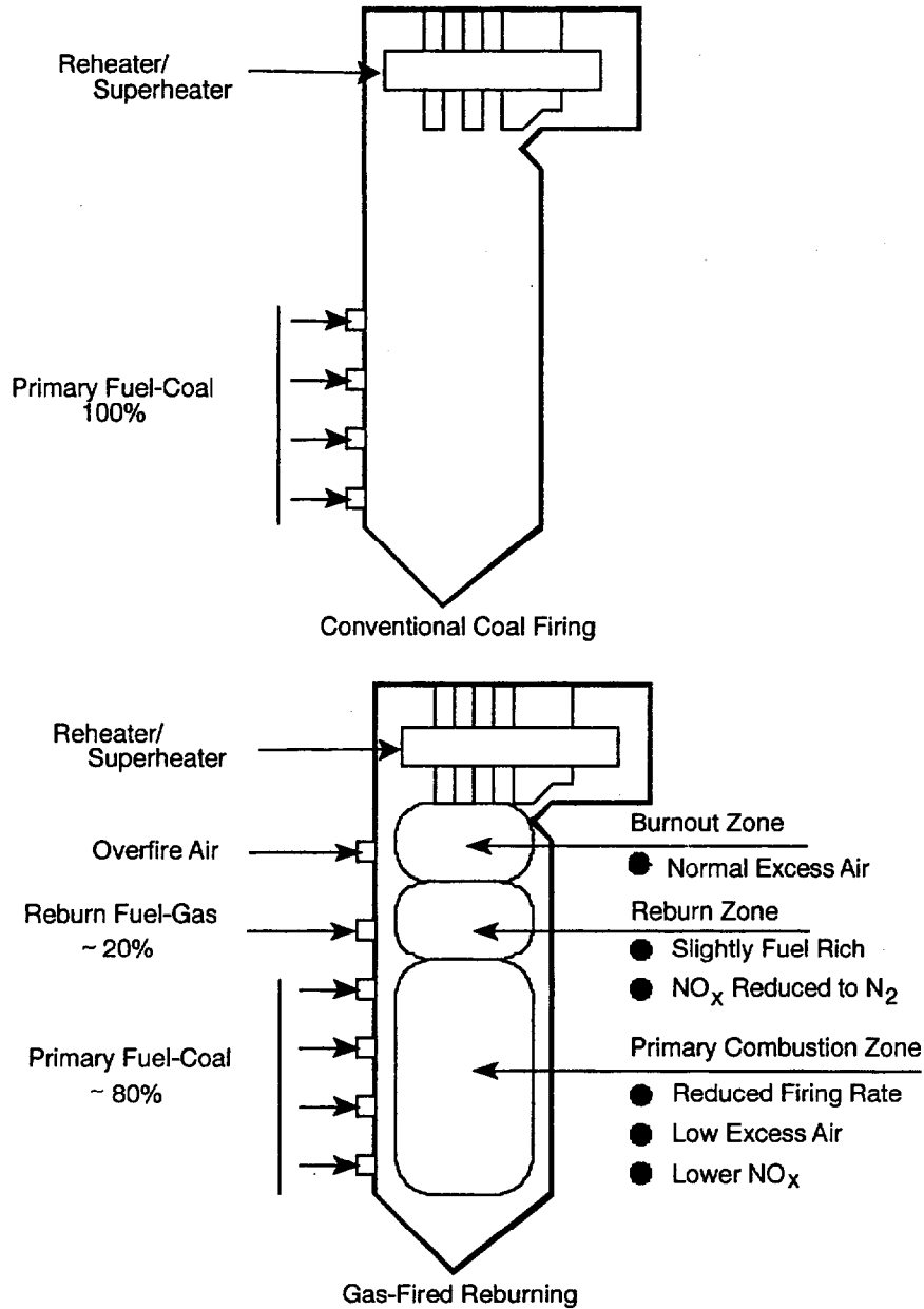
Figure 2-14. Conventional Firing and Gas-Fired Reburn Applied to a Wall-Fired Boiler (GRI, 1991).
