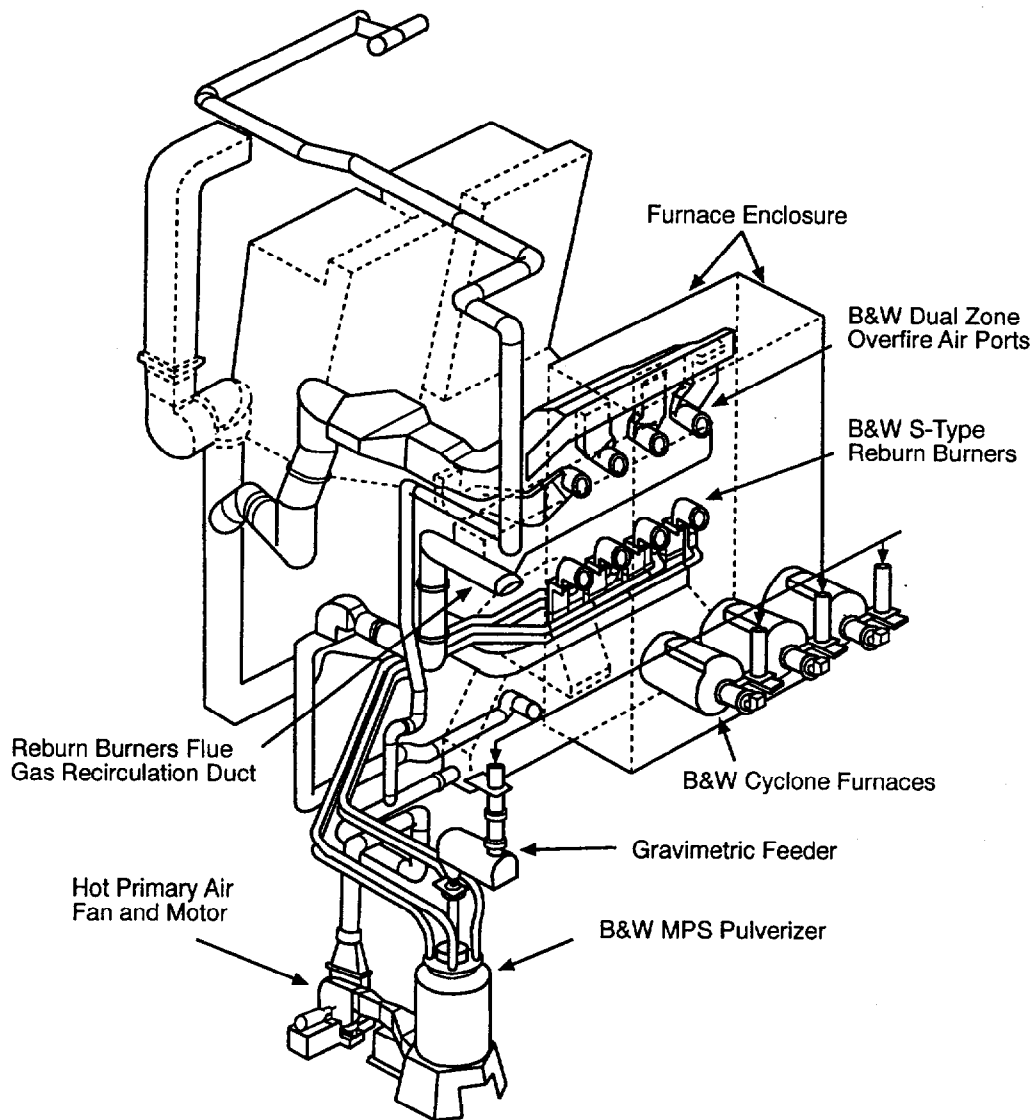
Figure 3-16. Nelson Dewey Unit 2—Coal-Fired Reburn System Schematic (Newell et al., 1993).
