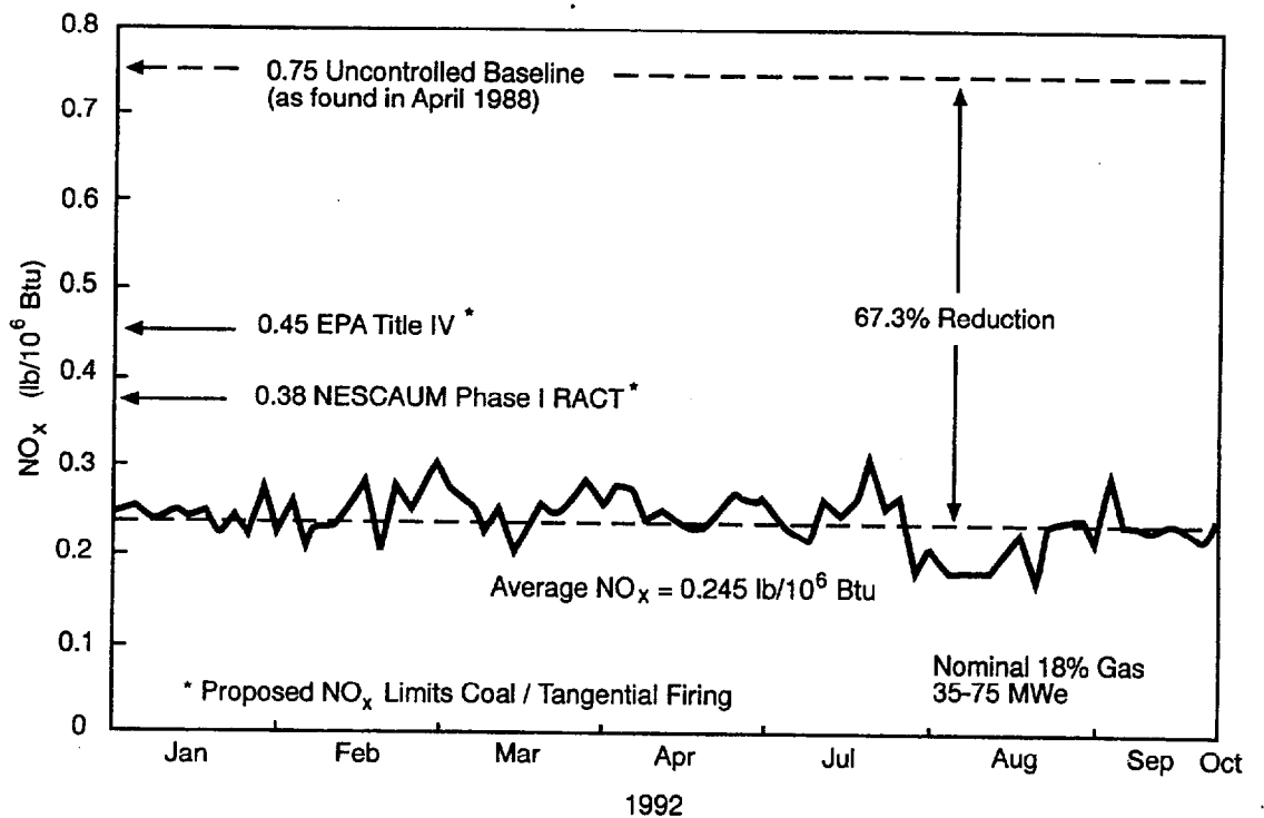
Figure 3-10. Hennepin Unit 1—Long-Term Gas Reburning Data (Folsom et al., 1993).
