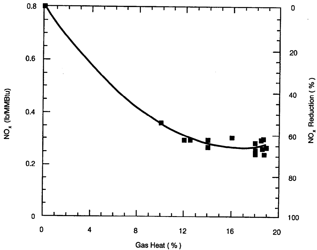
Figure 3-9. Hennepin Unit 1—Gas Reburning Data with Coal as the Primary Fuel (Folsom et al., 1993).
