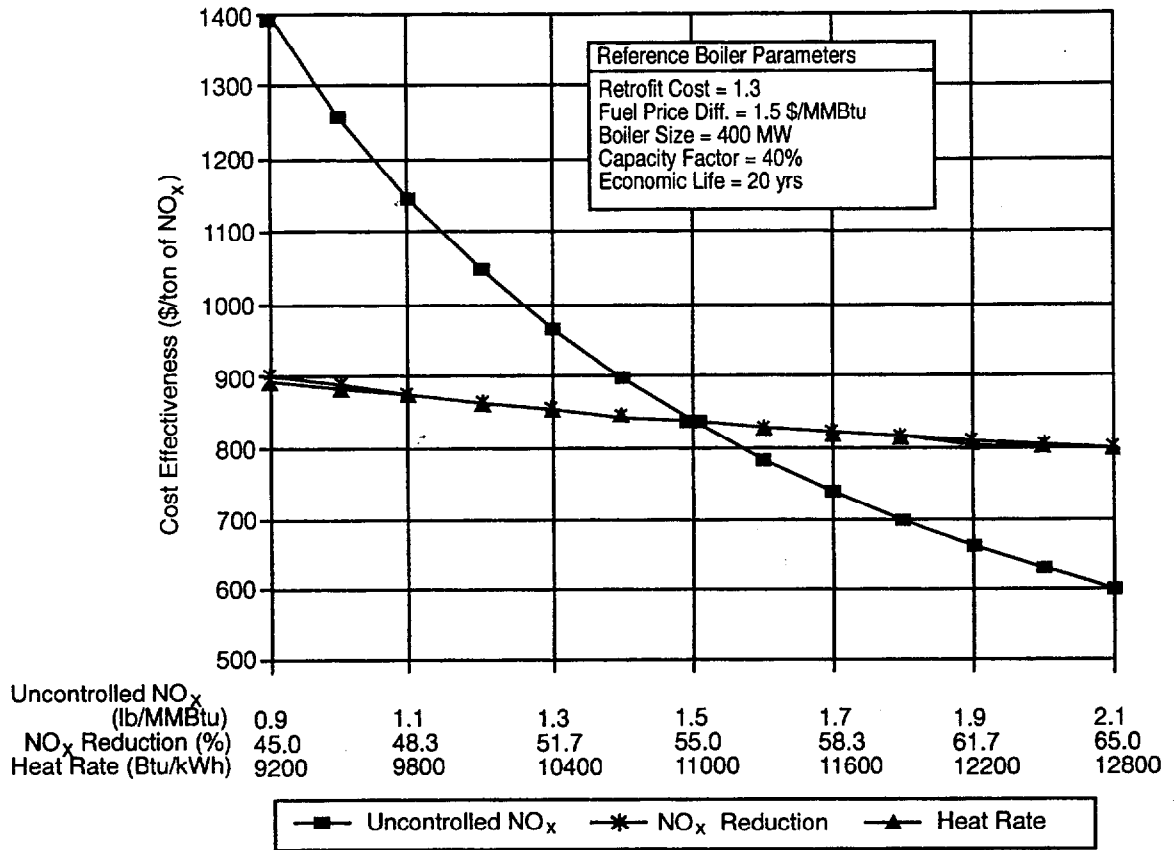
Figure 4-6. Impact of NO x Emission Characteristics and Heat Rate on Return Cost Effectiveness for Cyclone-Fired Boilers (U.S. EPA, 1994).
