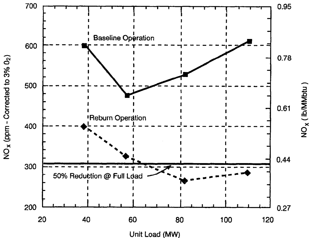
Figure 3-17. Nelson Dewey Unit 2-NO x Emissions vs. Unit Load - Illinois Basin Coal (Newell et al., 1993).
