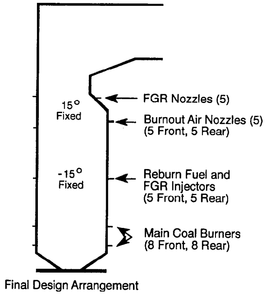
Figure 3-22. Ladyzhin Unit 4—Schematic of Reburn Design Arrangements (LaFlesh et al., 1993).
