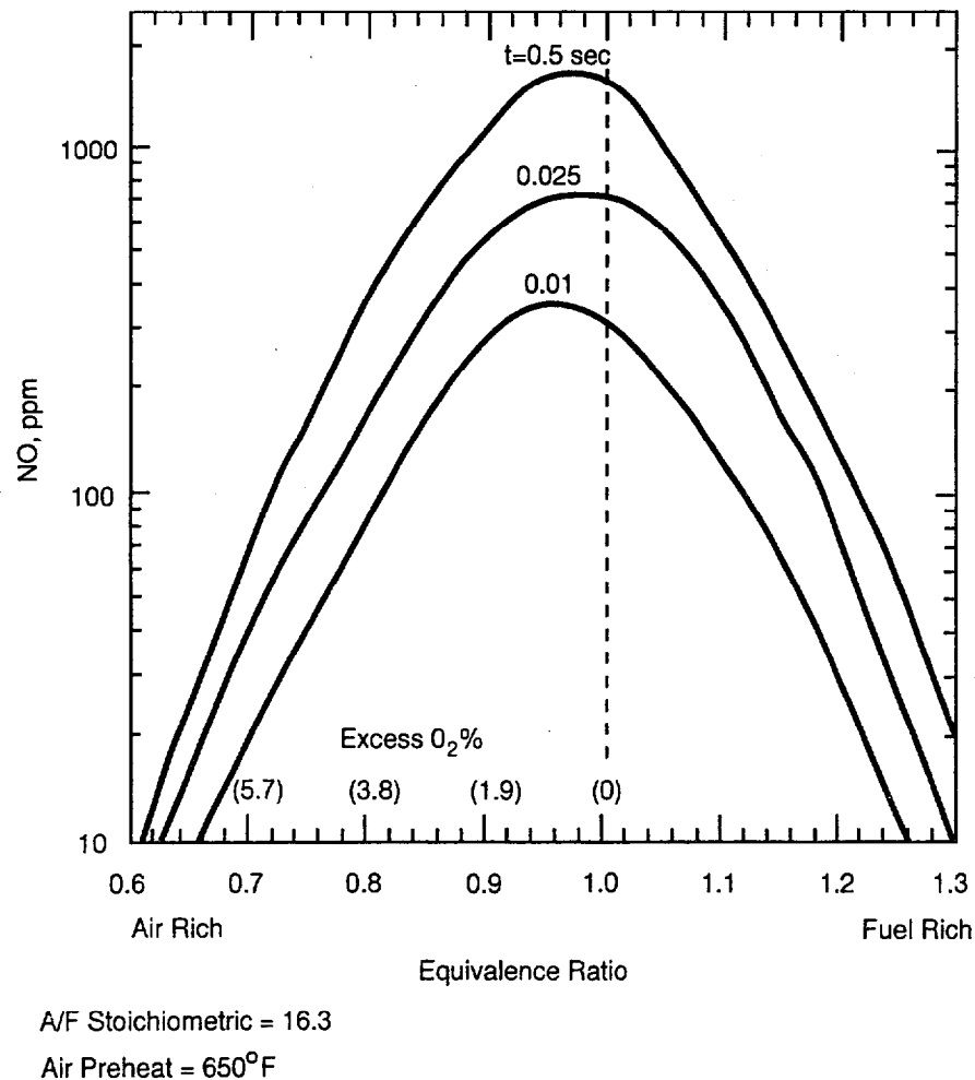
Figure 2-1. Effect of Equivalence Ratio on \text{NO}_x Formation (Bagwell, et al. 1971).
