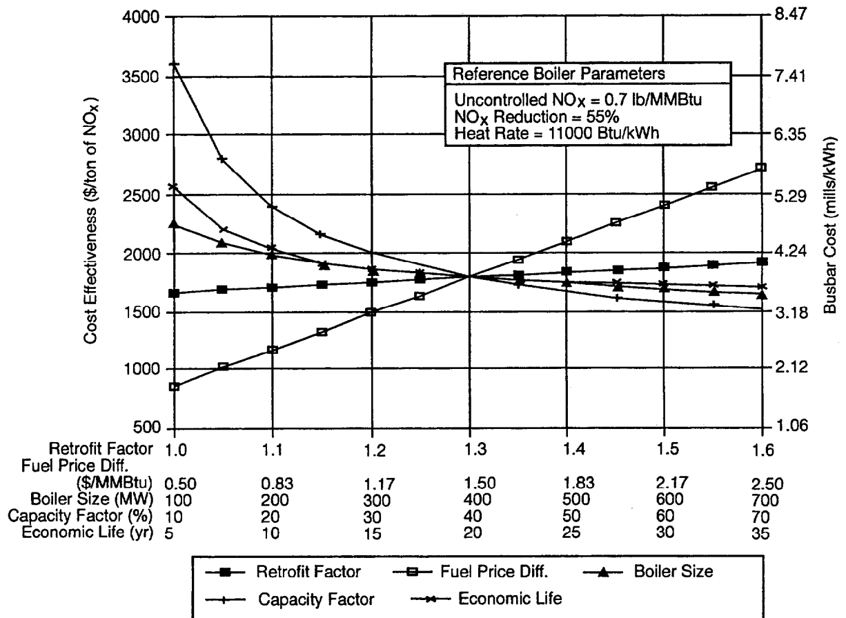
Figure 4-3. Impact of Plant Characteristics on Reburn Cost Effectiveness and Busbar Costs for Tangentially-Fired Boilers (U.S. EPA, 1994).
