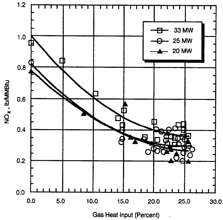
Figure 3-12. Lakeside Unit 7—Effect of Gas Heat Input on NO x Emissions (Folsom et al., 1994).
