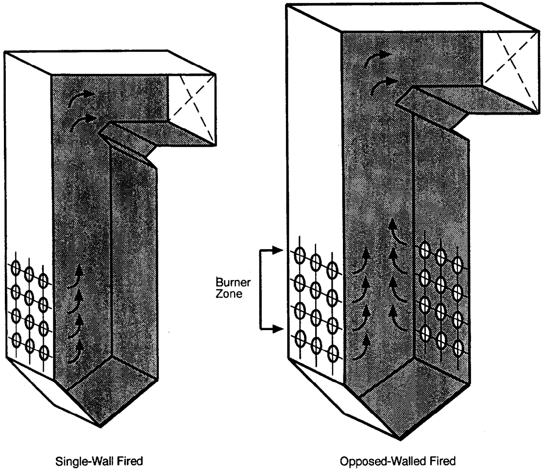
Figure 2-8. Single-Wall and Opposed-Wall Type Wall-Fired Boilers.
