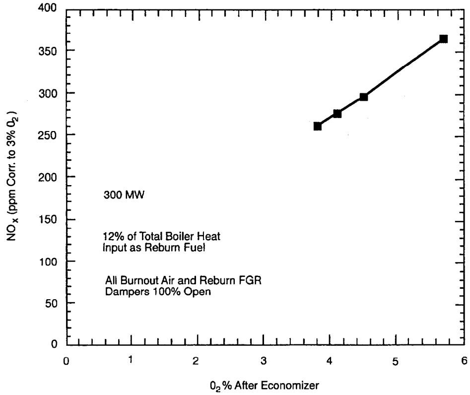
Figure 3-24. Ladyzhin Unit 4-NO x Emissions vs. Flue Gas Oxygen Content.
