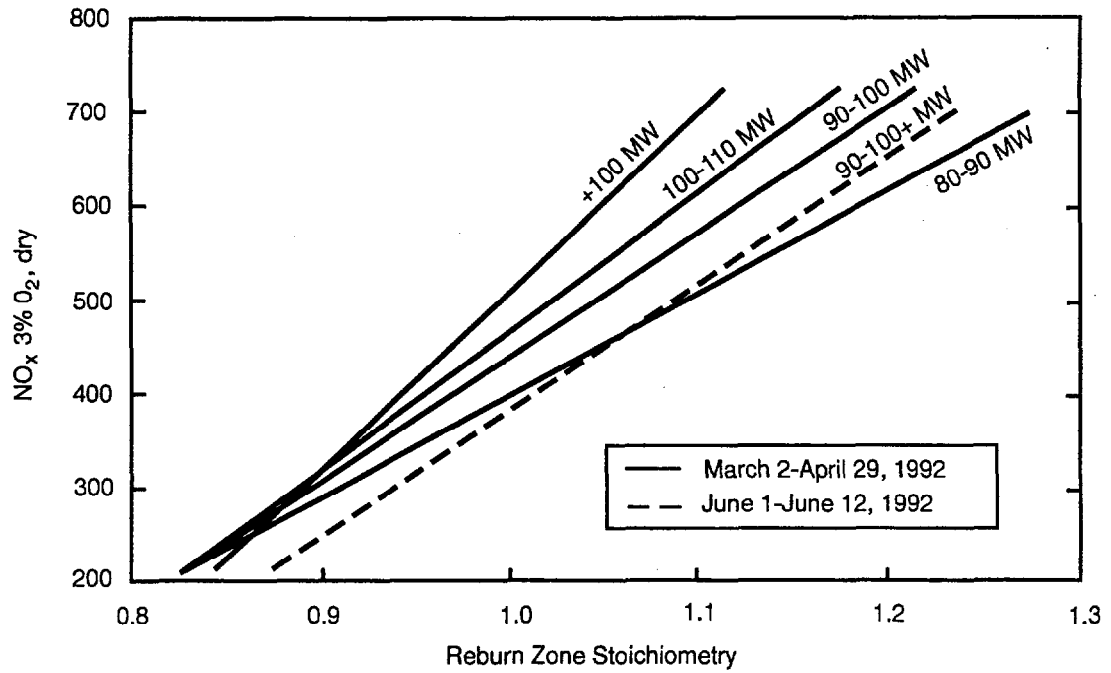
Figure 3-20. Niles Unit 1-Variation of NO x with Reburn Stoichiometry (Borio et al., 1993).
