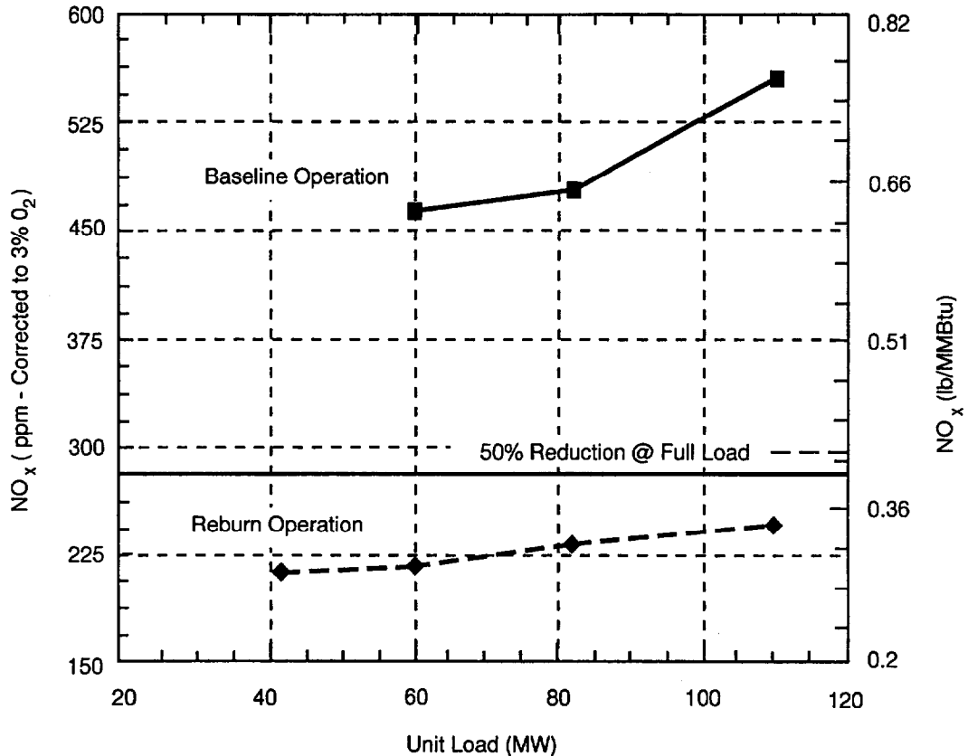
Figure 3-18. Nelson Dewey Unit 2-NO x Emissions vs. Unit Load - Powder River Basin Coal (Newell et al., 1993).
