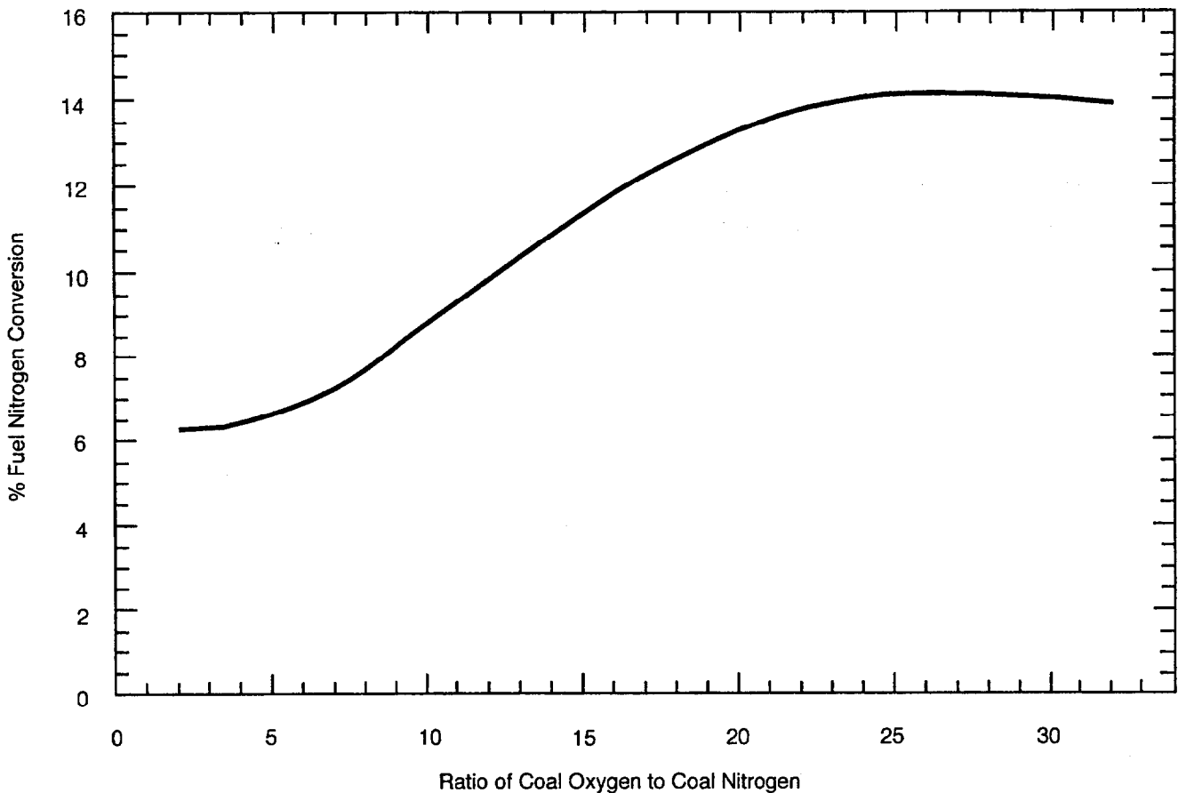
Figure 2-5. Fuel-Bound Nitrogen-to-Nitrogen Oxide in Pulverized Coal Combustion (Singer, 1991).
