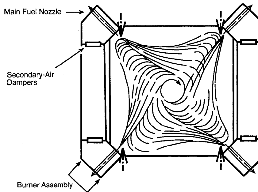
Figure 2-6. Firing Pattern in a Tangentially-Fired Boiler (Singer, 1991).
