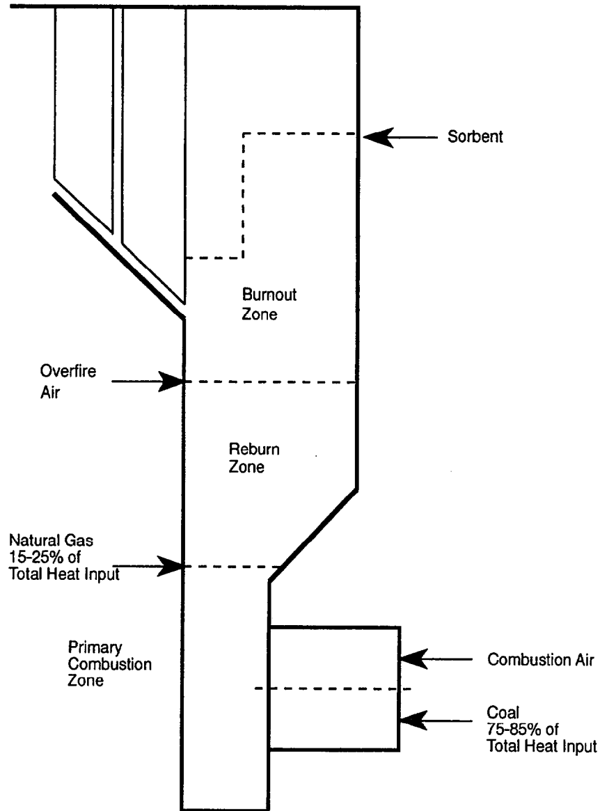
Figure 3-11. Lakeside Unit 7-GR-SI System Schematic (Folsom et al., 1994).
