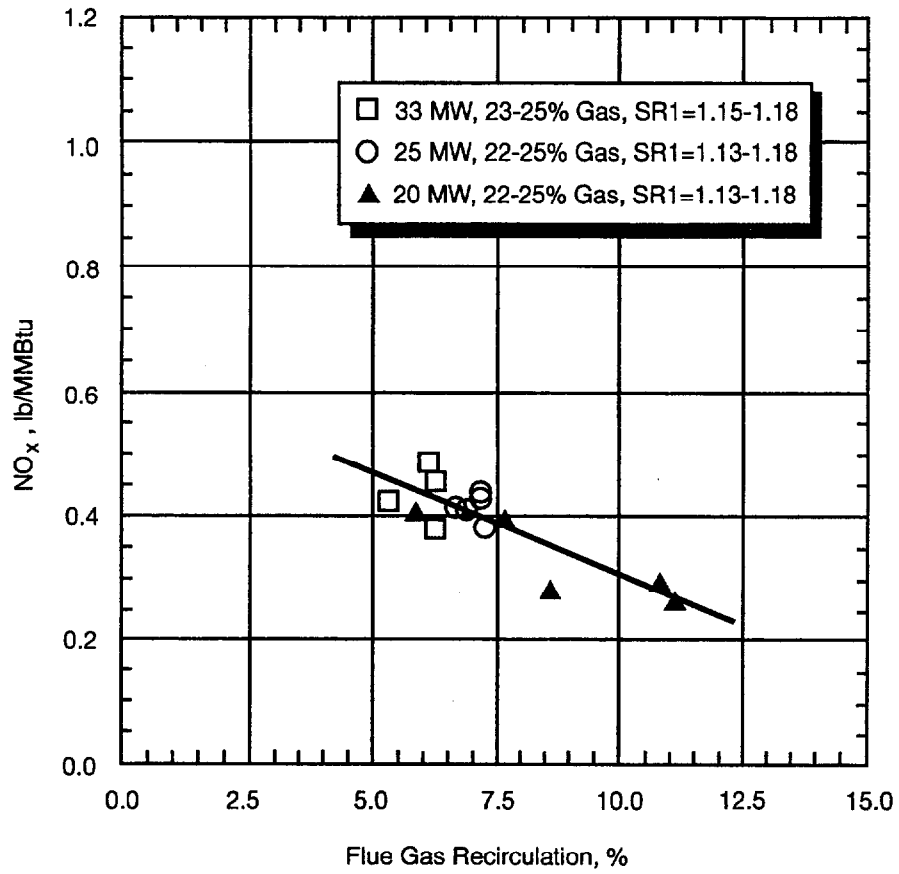
Figure 3-14. Lakeside Unit 7—Effect of Flue Gas Recirculation on NO x Emissions (Folsom et al., 1994).
