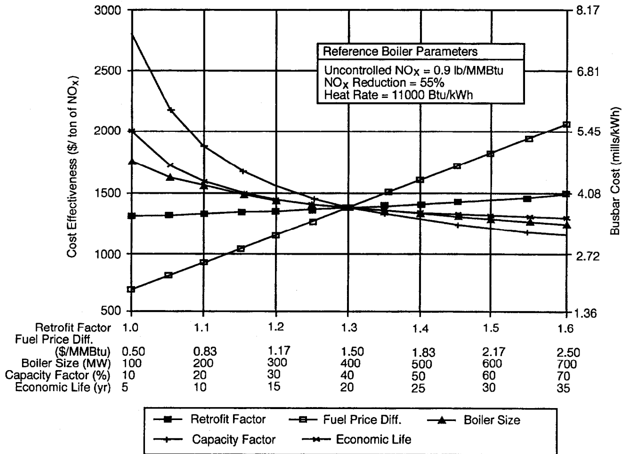
Figure 4-1. Impact of Plant Characteristics on Reburn Cost Effectiveness and Busbar Costs for Wall-Fired Boilers (U.S. EPA, 1994).
