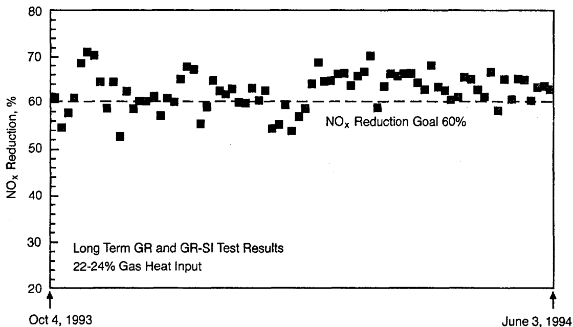
Figure 3-15. Lakeside Unit 7-Long-Term Operation Results for NO x Reductions (Folsom et al., 1994).
