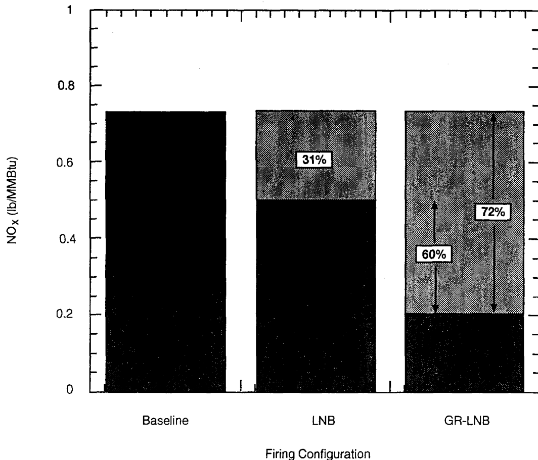
Figure 3-2. Cherokee Unit 3—Short-Term \text{NO}_x Emission Data (Sanyal et al., 1993).
