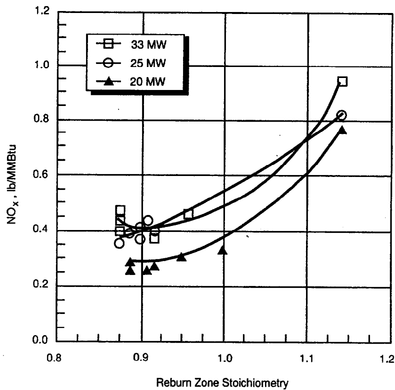
Figure 3-13. Lakeside Unit 7—Effect of Reburn Zone Stoichiometry on NO x Emissions (Folsom et al., 1994).
