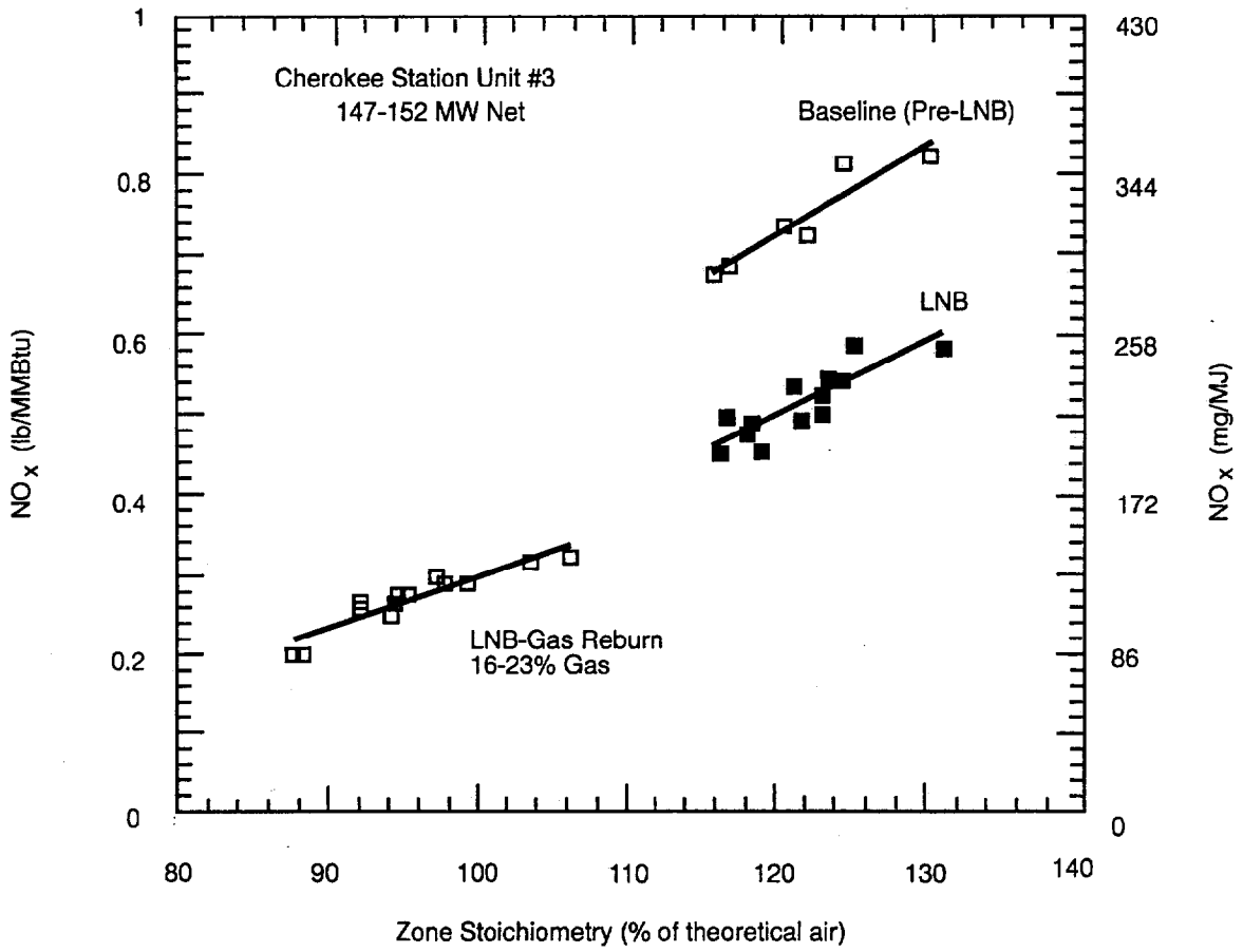
Figure 3-3. Cherokee Unit 3-LNB-Gas Reburning Data (Sanyal et al., 1993).
