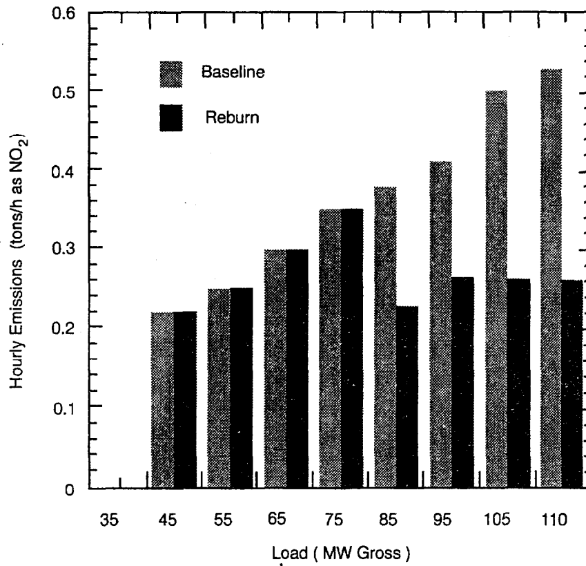
Figure 3-21. Niles Unit 1-NO x Emissions as a Function of Boiler Load (Borio et al., 1993).
