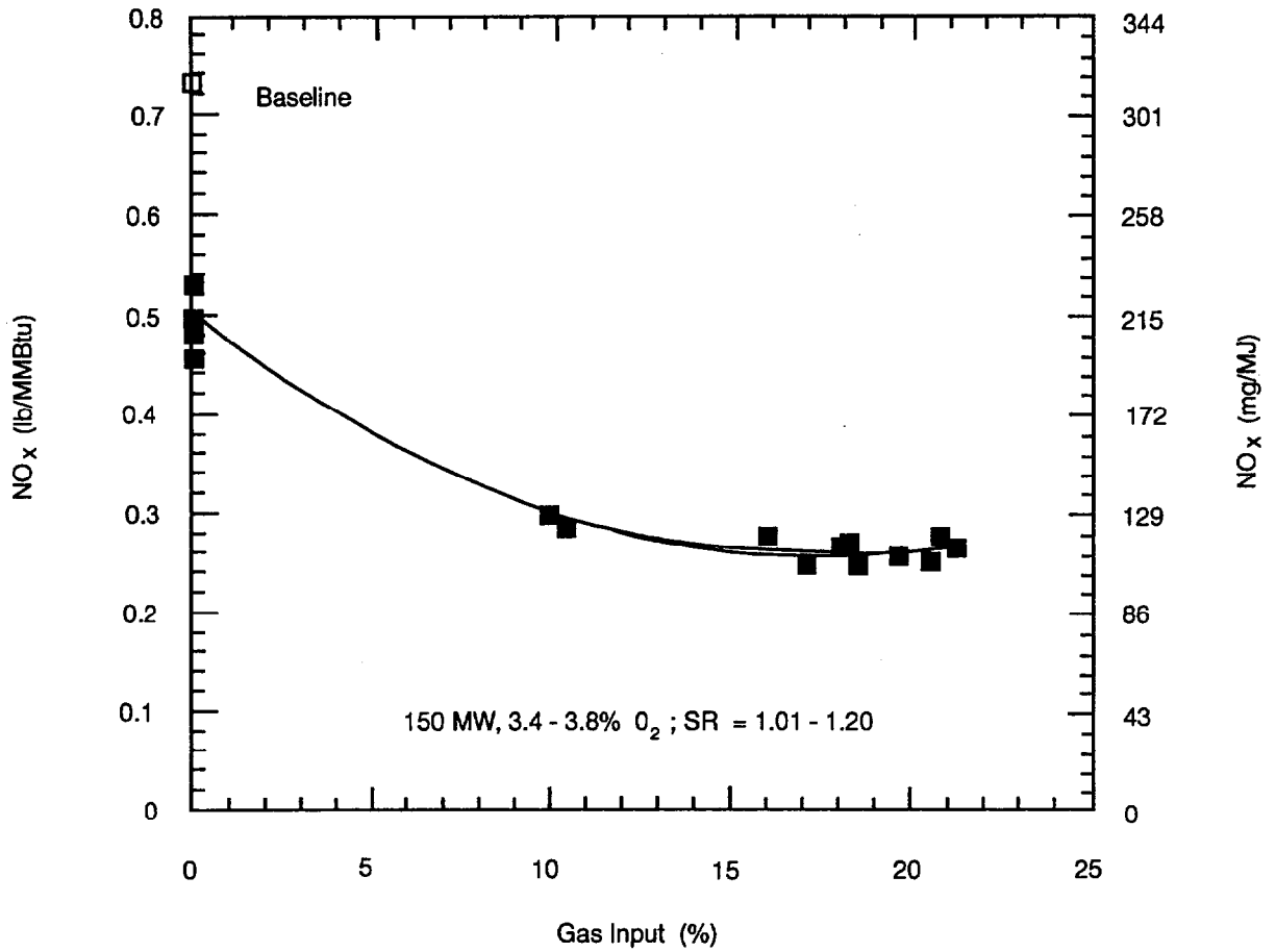
Figure 3-5. Cherokee Unit 3—Effect of Gas Input on NO x Emissions (Sanyal et al., 1993).
