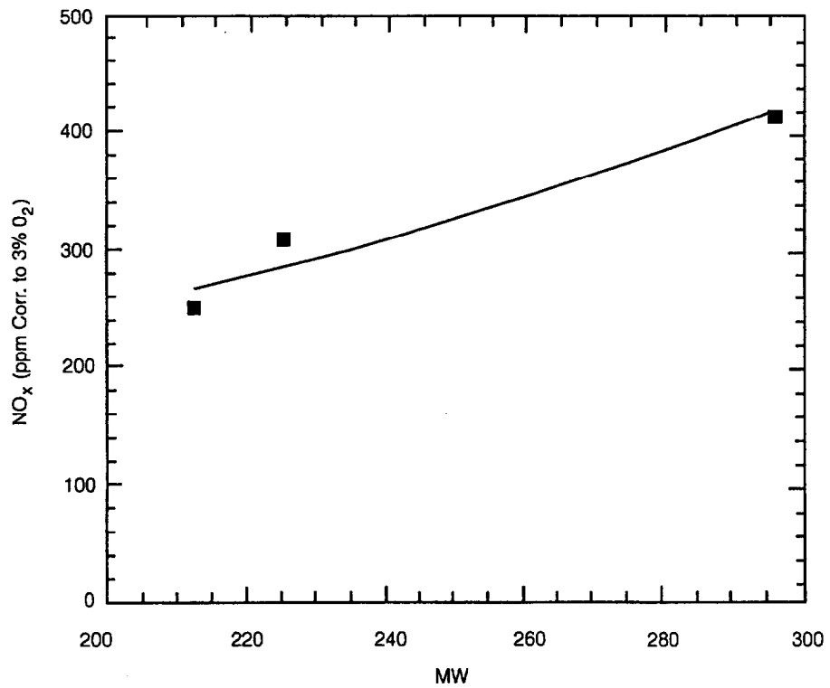
Figure 3-25. Ladyzhin Unit 4-NO x Emissions vs. Boiler Load.
