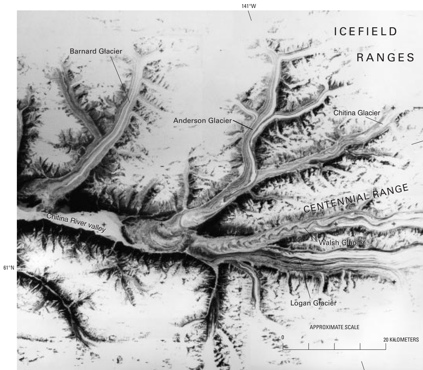
Figure 3. —Annotated enlargement of part of a Landsat 3 return beam vidicon (RBV) image showing the glaciers of the upper Chitina River valley basin, St. Elias Mountains, Yukon Territory-Alaska. Walsh Glacier shows well-defined moraine loops that identify the glacier as surging. Its 1960–64 surge displaced ice as much as 11.5 km—a record for North America. The approximate 1968 surge of Anderson Glacier truncated the terminus of Chitina Glacier, another surging glacier. Logan Glacier is not included in Post's (1969) catalog of surging glaciers; the moraine loops near its confluence with Walsh Glacier indicate variations in flow velocity, but these may be in response to surges of Walsh Glacier. The Landsat 3 RBV image (30853–19510; 5 July 1980; Path 68, Row 17, Subscene C) is archived by the U.S. Geological Survey Glacier Studies Project. Map references: Kluane Lake map sheet 115G and 115F (E 1/2); Mount St. Elias map sheet 115B and 115C; Bering Glacier map sheet N6000–W14100/60x180; McCarthy map sheet N6100–W14100/60x180; all 1:250,000 scale.
