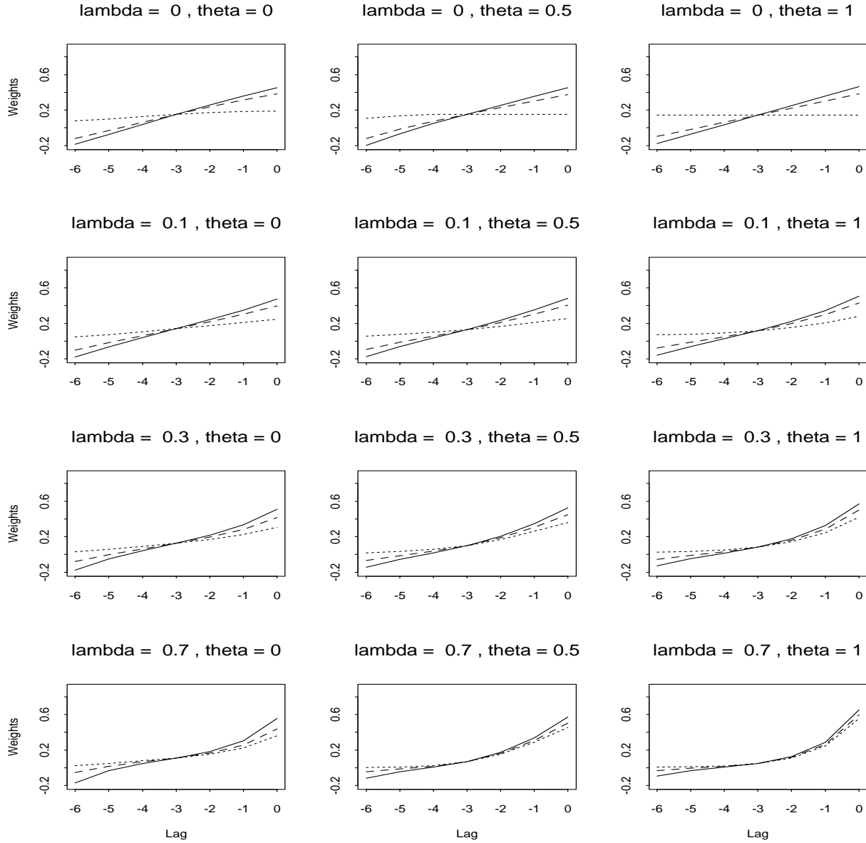
Figure 13: Plots of the impulse response functions of the BLIP end filters for q = 0 based on the local linear model ( p = 1 ) and the 13 point central filters given by Theorem 1. These end filters are evaluated for selected values of \theta and \lambda . The solid lines correspond to \hat{\beta}_p^2 / \hat{\sigma}^2 = \infty (this yields the BLUP end filters), the dashed lines to \hat{\beta}_p^2 / \hat{\sigma}^2 = 4 / (\pi(3.5)^2) (this value gives the X-11 end filter in the case where p = 1 , \lambda = 0 and the central filter concerned is the X-11 13 point Henderson filter), and the dotted lines to \hat{\beta}_p^2 / \hat{\sigma}^2 = 0 . When \beta_p^2 = 0 the latter choice for \hat{\beta}_p^2 / \hat{\sigma}^2 corresponds to the BLUP end filter for the reduced model of order p - 1 and represents the best mean squared revisions possible.
