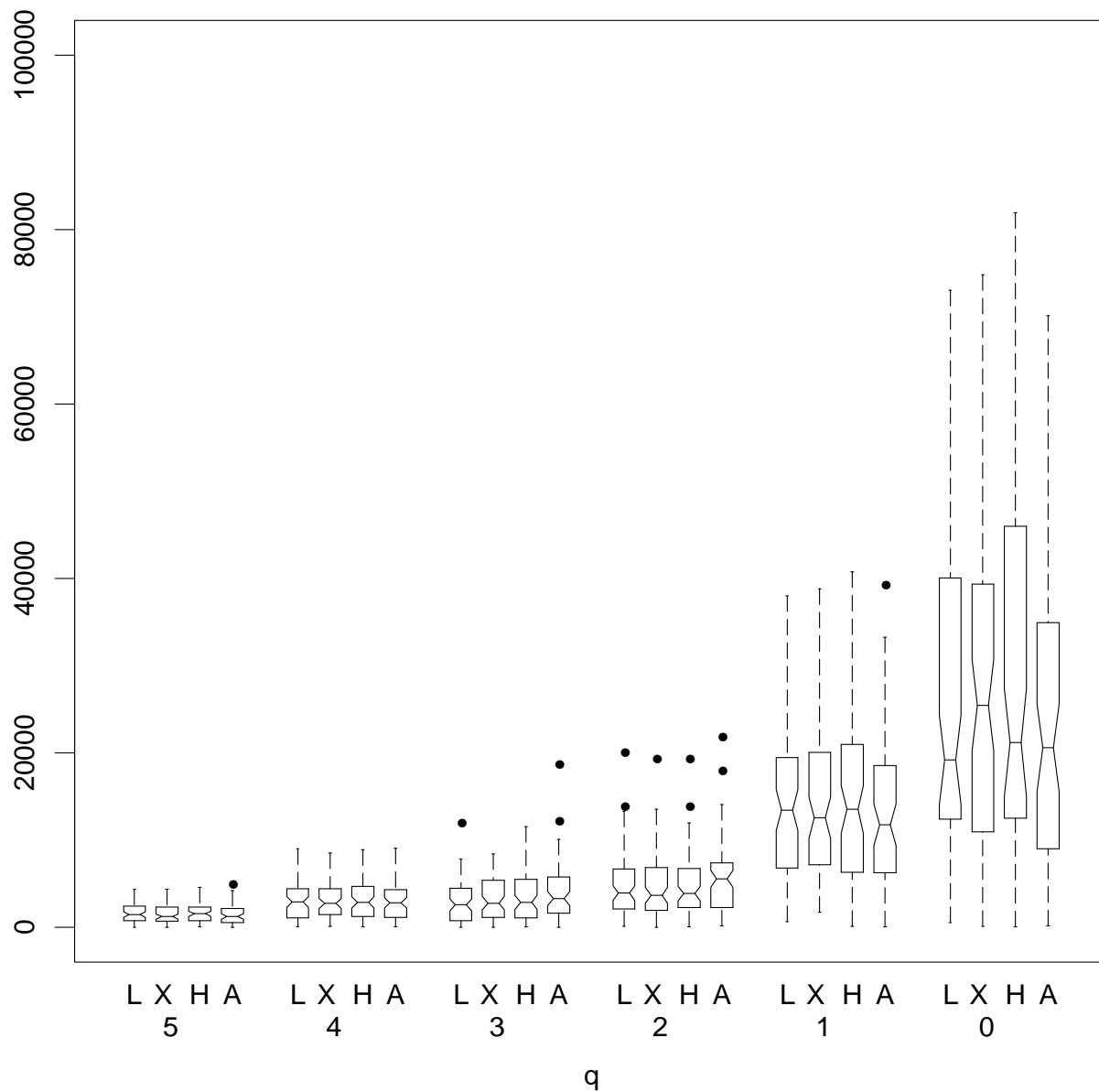
Figure 37: Merchandise Exports data. Using the central X-11 Henderson filter in the body and the local linear model, comparisons are made between the various end filters and for the various values of q . The choice of \lambda = 0.52 is determined by searching for values which improve the revisions for the BLUP end filter for the q = 0 case. The choice of \hat{\beta}_p^2/\hat{\sigma}^2 = 0.30 is determined by searching for values which improve the revisions given \lambda . Here L refers to the BLIP end filter based on the local linear model and the choices of \lambda and \hat{\beta}_p^2/\hat{\sigma}^2 given above. Likewise, X refers to the standard X-11 end filter and H refers to the BLUP end filter based on the local linear model. Note that the X-11 end filters are BLIP end filters based on the central X-11 Henderson filter, a local linear model with \lambda = 0 and \hat{\beta}_p^2/\hat{\sigma}^2 = 4/(\pi(3.5)^2) or .104. Finally A refers to the filter obtained by using the central filter with unknown observations predicted by a global ARIMA model.
