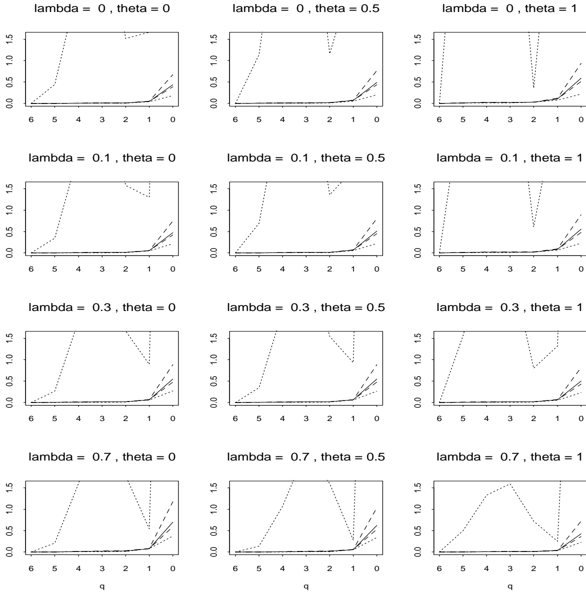
Figure 19: Plots of the mean squared revisions criterion R_q(\hat{\phi}_0) for the BLIP end filters based on the local quadratic model ( p = 2 ), the optimum central filters given by Theorem 1 and selected values of \theta and \lambda . Here the solid line corresponds to \hat{\beta}_p^2/\hat{\sigma}^2 = \infty (this yields the BLUP end filters), the dashed lines to \hat{\beta}_p^2/\hat{\sigma}^2 = 4/(\pi(3.5)^2) (this value gives the X-11 end filter in the case where p = 1 , \lambda = 0 and the central filter concerned is the X-11 13 point Henderson filter), and the dotted lines to \hat{\beta}_p^2/\hat{\sigma}^2 = 0 (this value gives the BLUP end filter for the reduced model of order p - 1 ). In each case the mean squared revisions are plotted for the \beta_p^2/\sigma^2 = 0 (lower limit) and \beta_p^2/\sigma^2 = 4/\pi (upper limit). Since it is unbiased, the mean squared revisions for the BLUP end filter do not depend on the choice of \beta_p^2/\sigma^2 .
