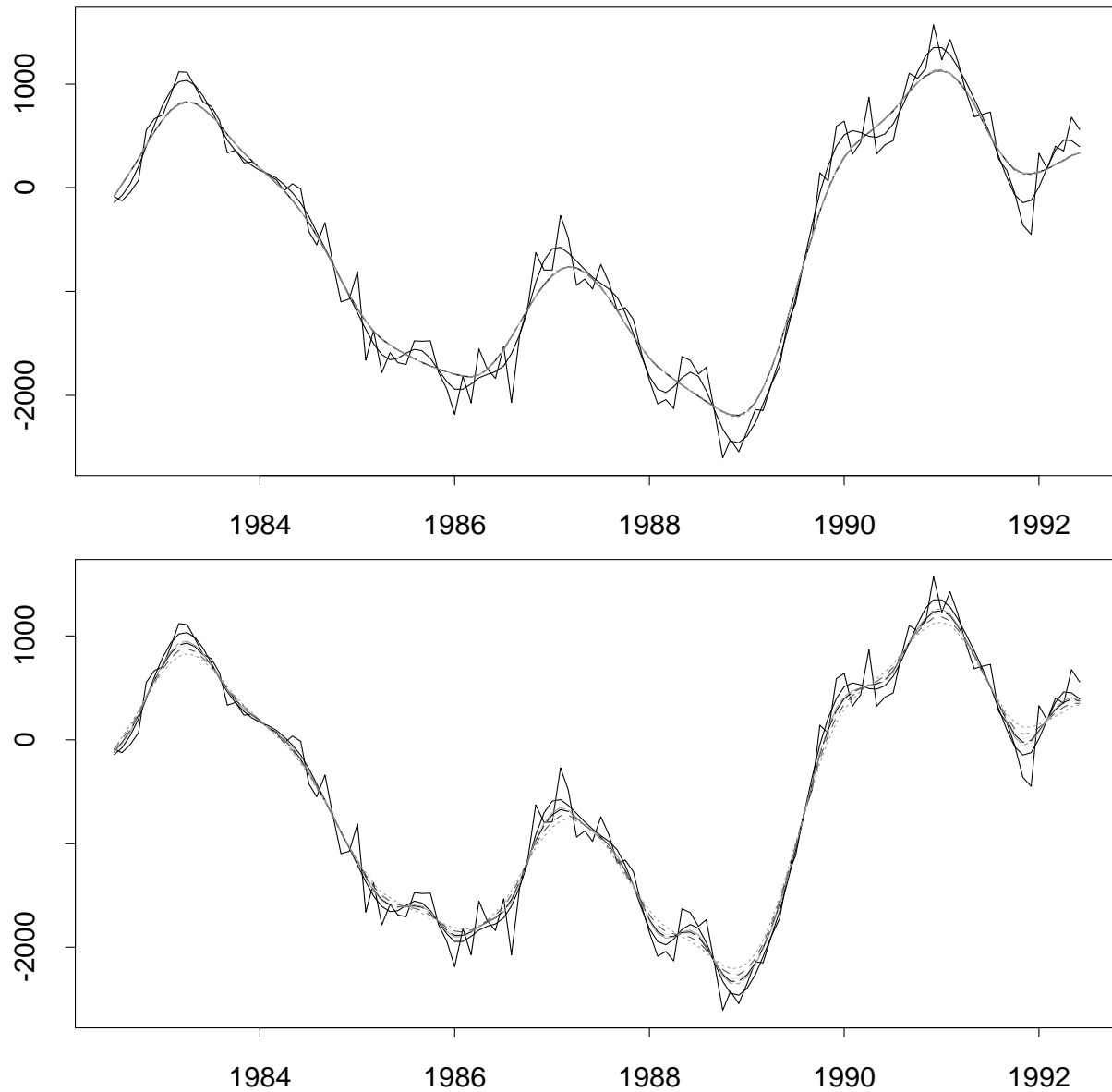
Figure 34: The Permanent Migration data is characterised by many local turning points, with almost zero drift long term. In the top graph, the data is filtered by the 13 point X-11 Henderson filter and the 13 point filters given by Theorem 1 for the local linear model and \theta = 0 . In the bottom graph, the data is filtered by the 13 point X-11 Henderson filter and the 13 point filters given by Theorem 1 for the local linear model and \theta = .5 . In both graphs, the solid line corresponds to the 13 point X-11 Henderson filter, the dotted and dashed lines to the 13 point filters given by Theorem 1 with \lambda = .1, .2, .3, .4, .5 respectively.
