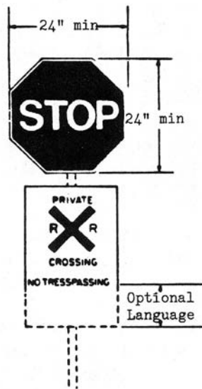
Figure 68. Typical Private Crossing Sign
