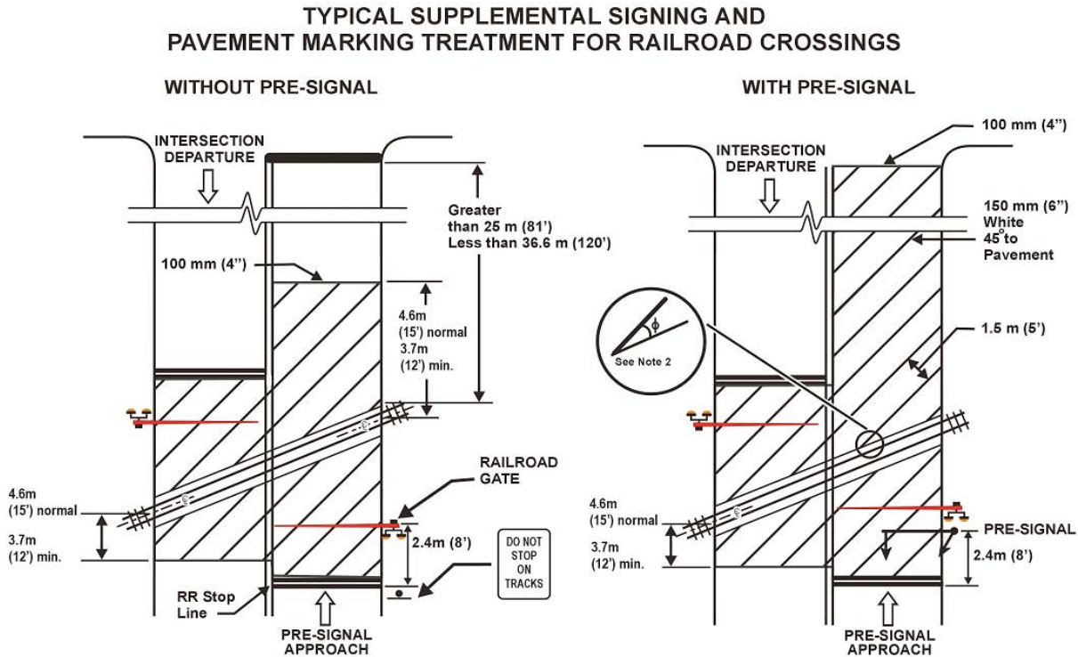
Figure 21. Typical Supplemental Signing and Pavement Marking Treatment for Railroad Crossings
