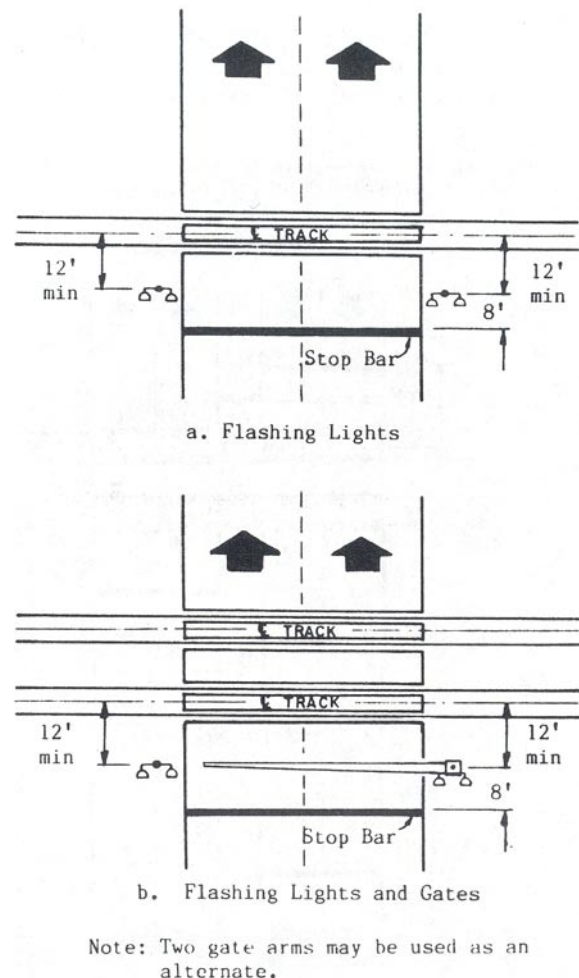
Figure 30. Typical Location Plan, Right Angle Crossing, One-Way, Two Lanes
