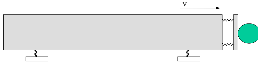
Figure A-26. Schematic of Lumped-Mass CD Model
