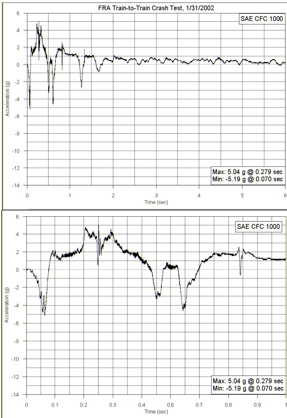
Figure D-3: Experiment No. 1-1 M-Style Seat, Aft Row, Aisle Seat, Hybrid III 50 th Head Z-axis Acceleration
