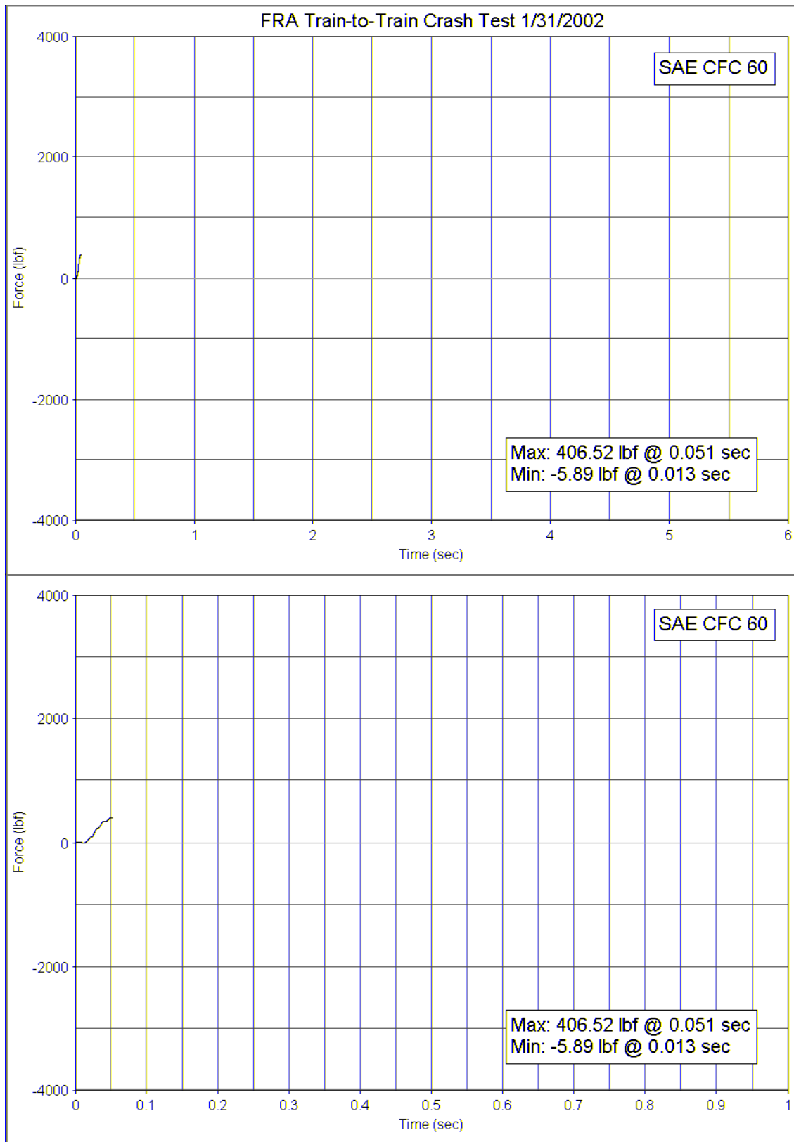
Figure C-11: Experiment No. 1-1 M-Style Seat, Forward Row, Right Rear Leg, Y-Axis Force
