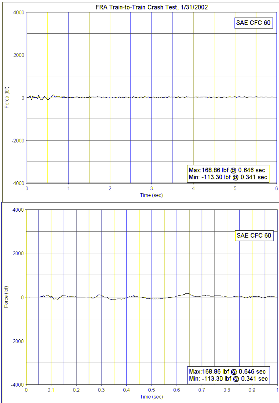
Figure C-35: Experiment No. 2-2 M-Style Seat, Forward Row, Left Rear Leg, Y-Axis Force
