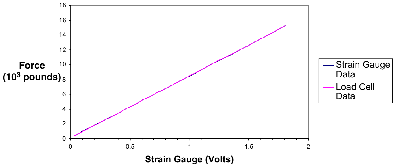
Figure A-7. Tangent east vertical crib No. 2
