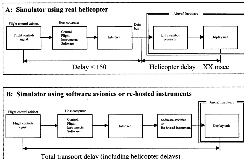
Figure C2HA and C2HB Transport delay for simulation of helicopters using real or re-hosted instrument drivers
