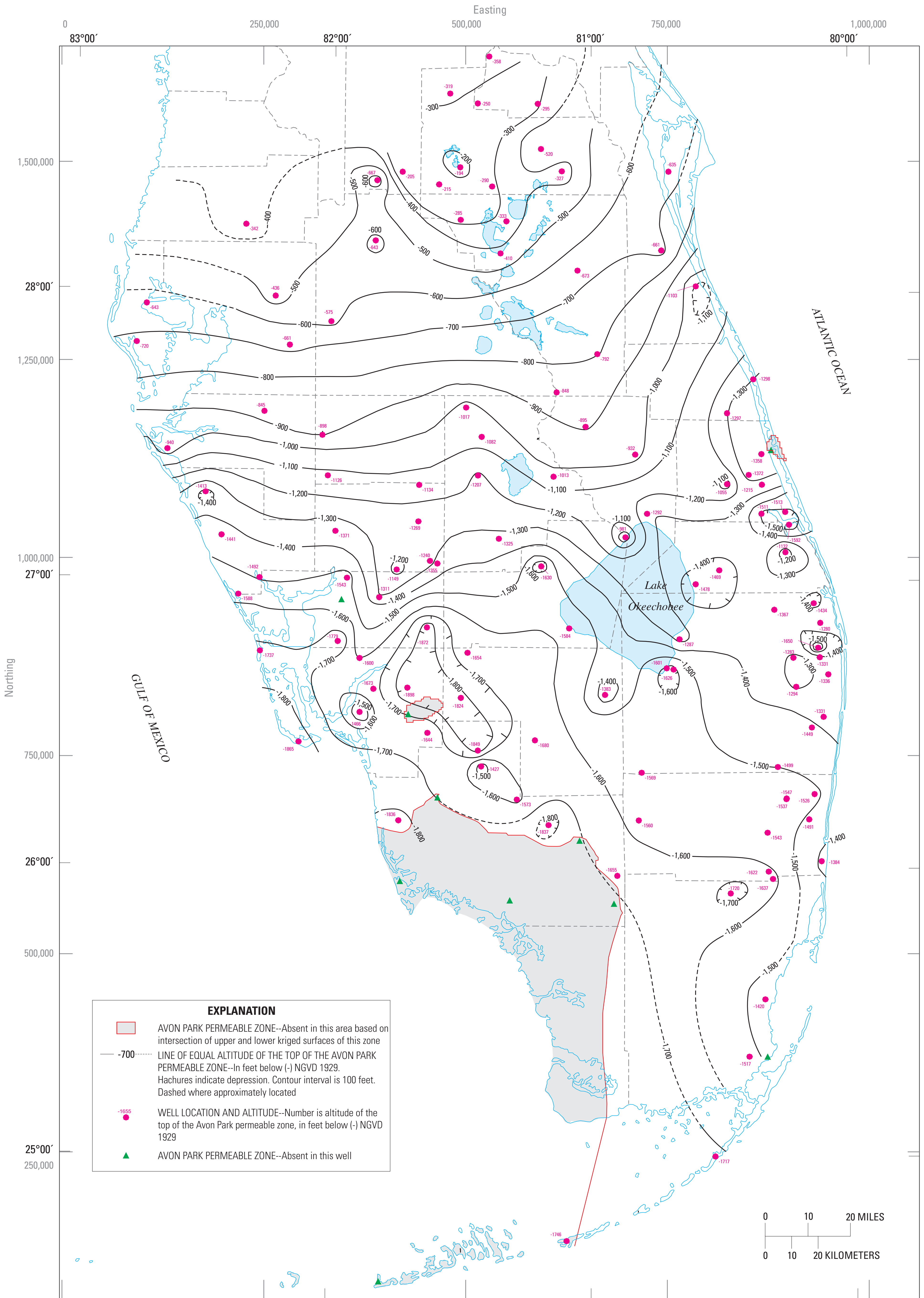
Figure A8. Altitude of the top of the Avon Park permeable zone in the Floridan aquifer system.
