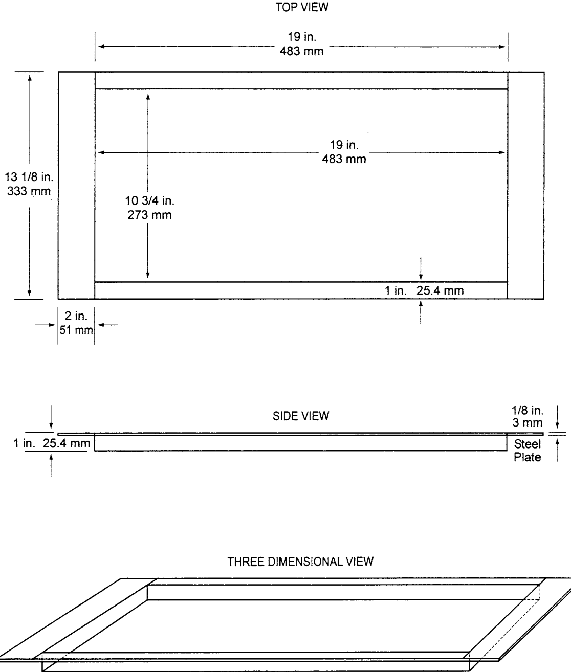
Figure 5: 3 views
