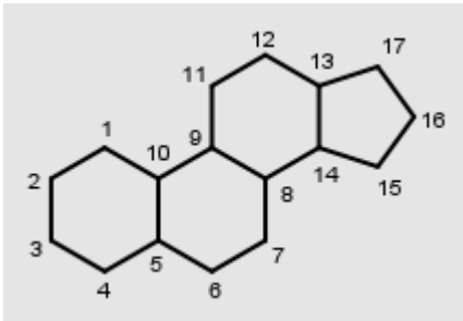
General chemical structure
