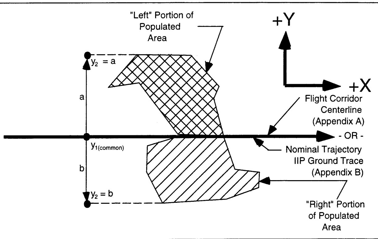
Figure C-4: Flight Azimuth Intersecting a Populated Area
