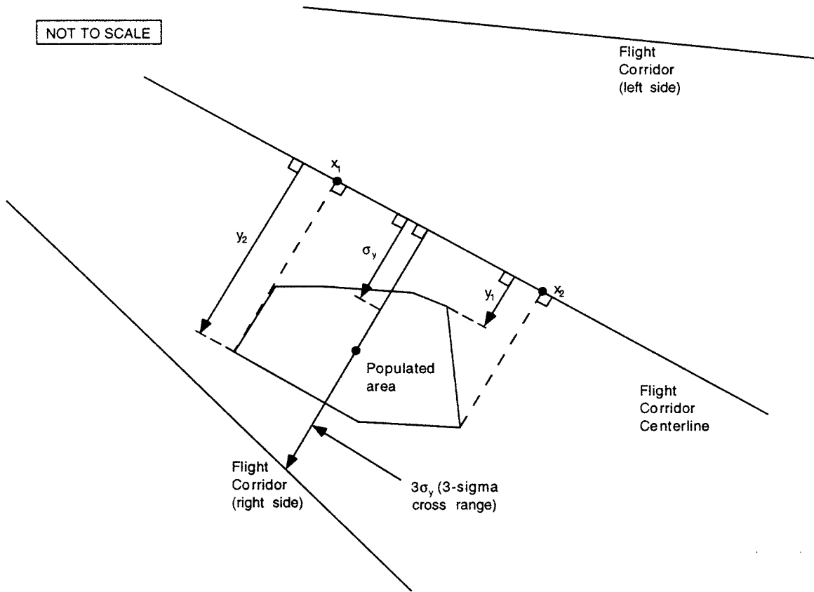
Figure C-1: Analysis of an Appendix A Flight Corridor
